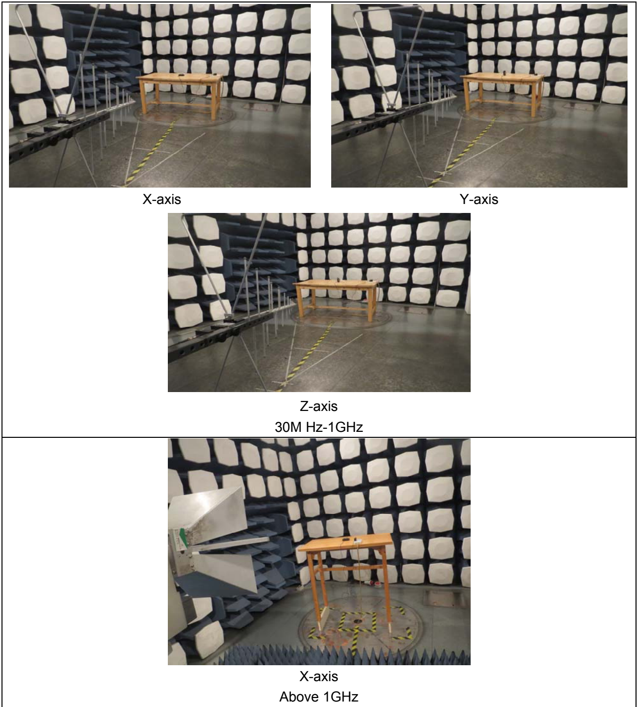
Picture 2 Radiated Emission Test Setup
