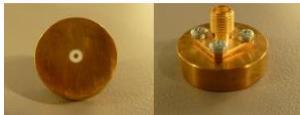
Figure 1 – MVG LIMESAR Dielectric Probe
