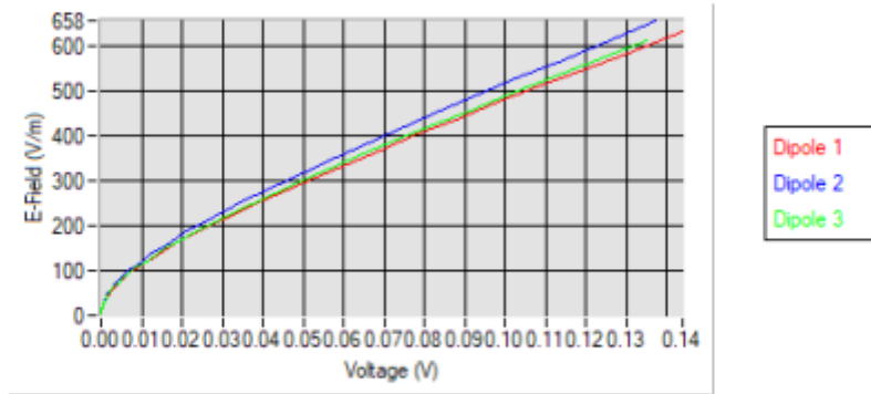
Calibration curves
