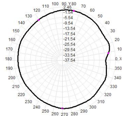
Efficiency:62.7%
