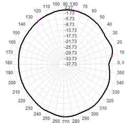
Efficiency:64.85%
