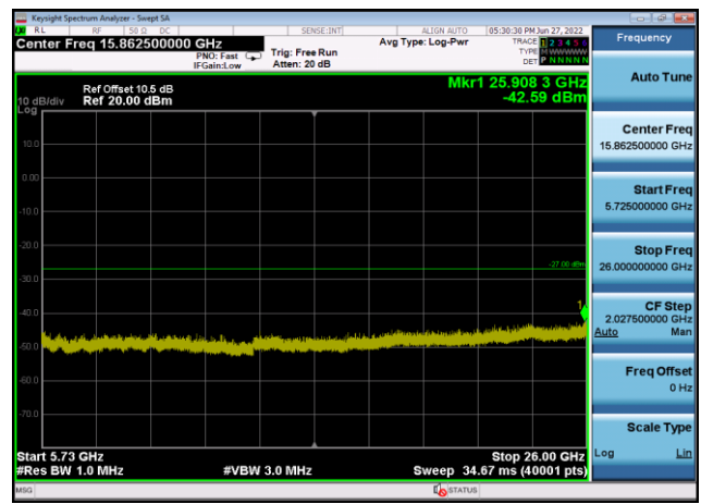
U-NII-2c ,Plot 3,5725MHz~26000MHz-802.11a(20MHz),5600MHz,Ant1
