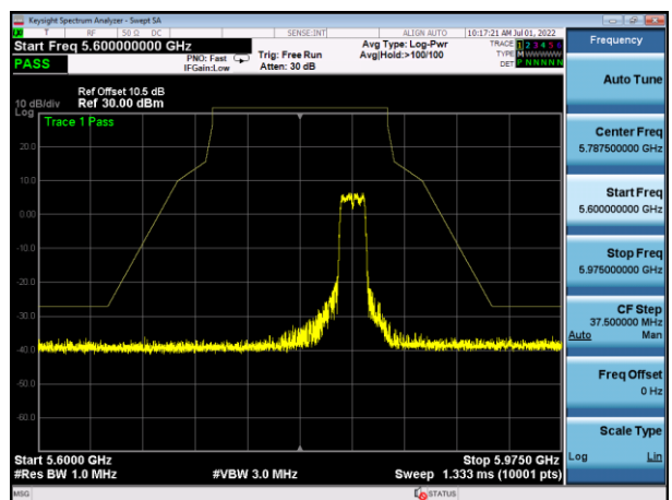
U-NII-3 ,Plot 1,Band Edge-802.11ac(20 MHz),5825MHz,Ant1
