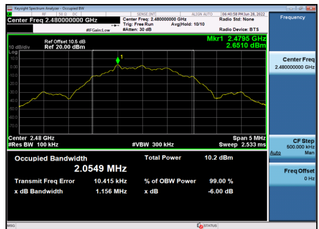
2MHz - 6dB Bandwidth: 2480MHz
