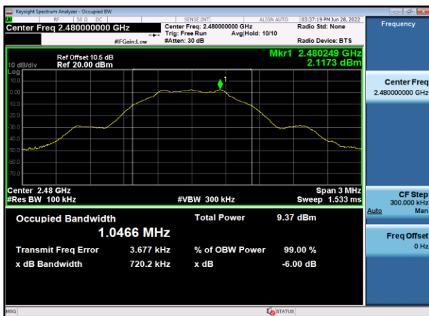
1MHz - 6dB Bandwidth: 2480MHz
