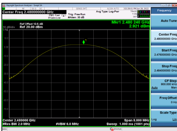
1MHz -Output Power: 2480MHz
