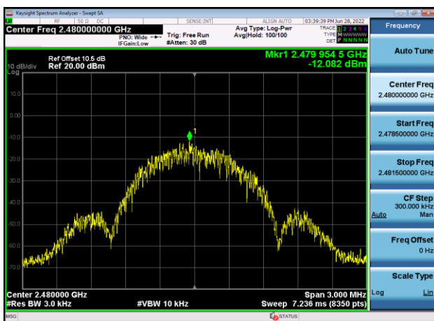
1MHz -Power spectral density: 2480MHz
