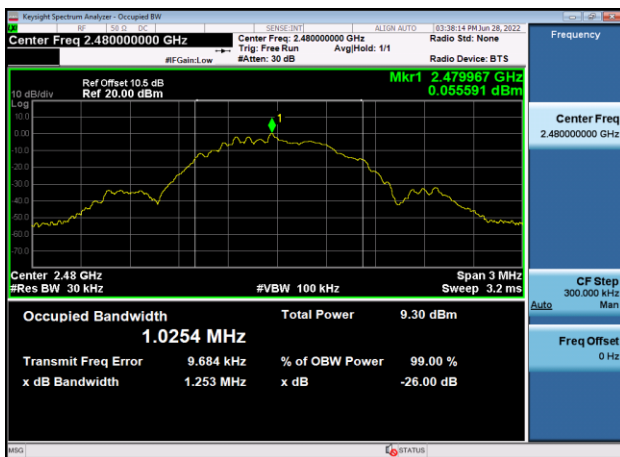
1MHz - 99% Bandwidth: 2480MHz
