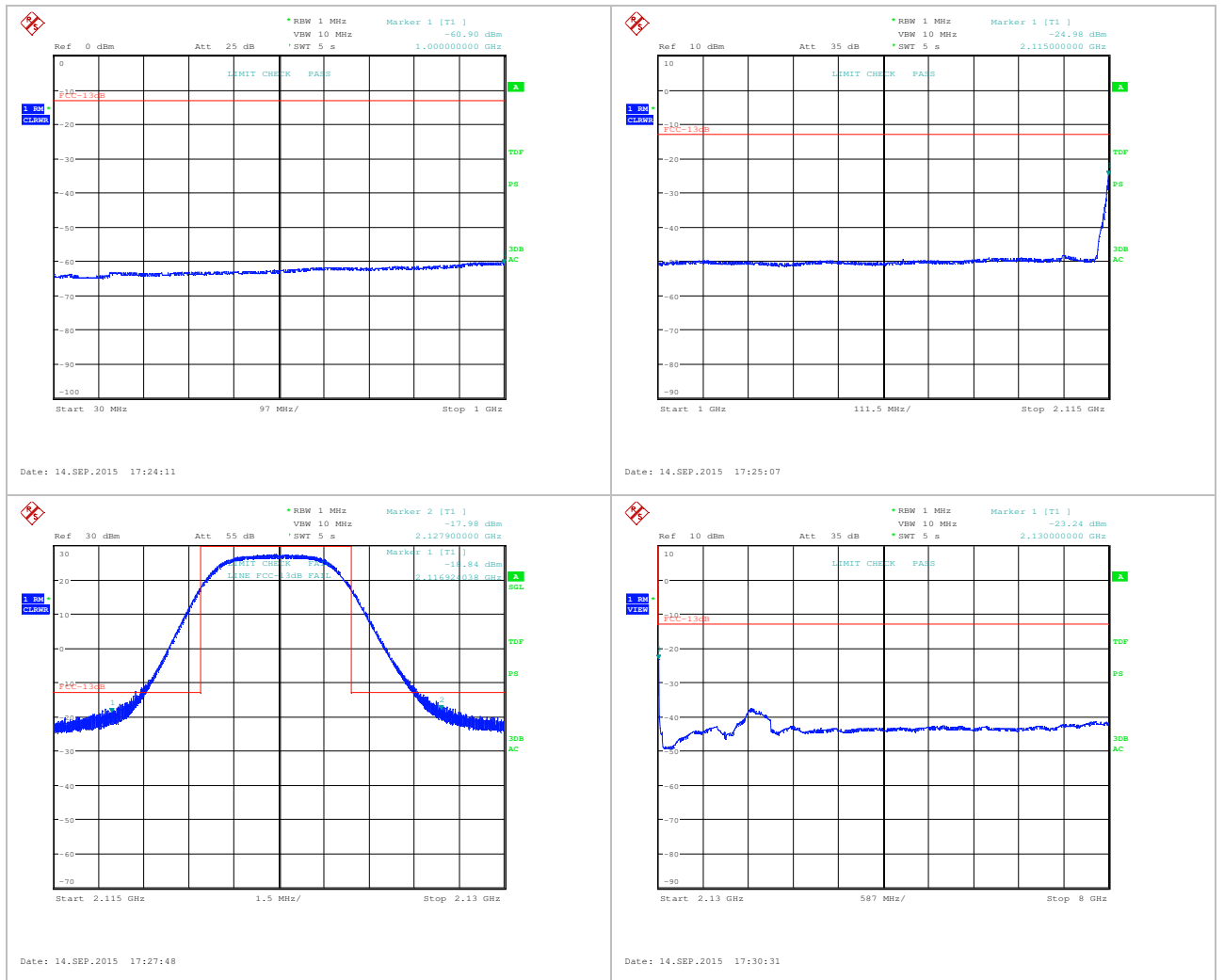
Figure 8: CSE plots: Ch 1587: 16QAM
