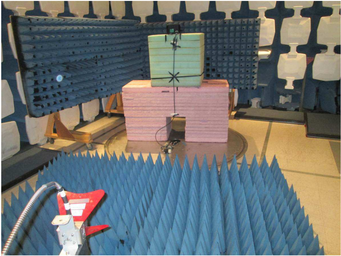
Radiated Emissions – 1 to 6 GHz
