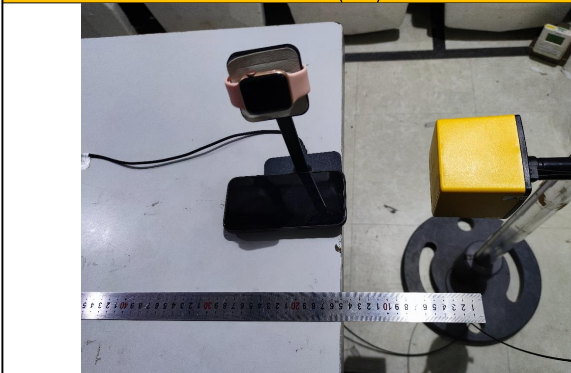
E-Field Strength and H-Field Strength Position A (15cm)
