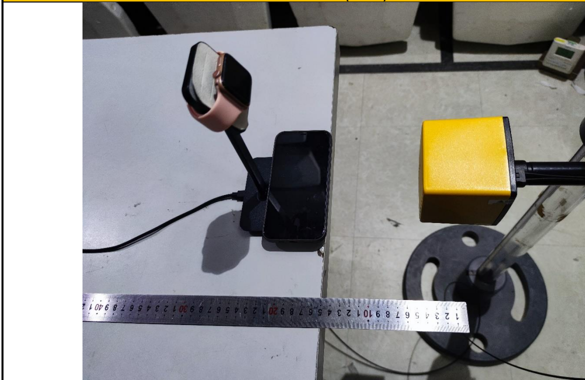
E-Field Strength and H-Field Strength Position C (15cm)
