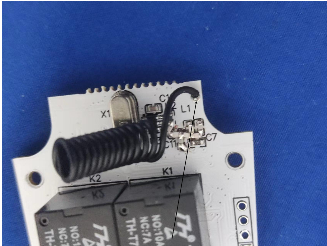
Spring antenna
