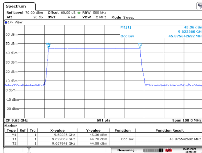
Figure 8.3-9: 99% bandwidth, tx on high channel with sweeping turned on
