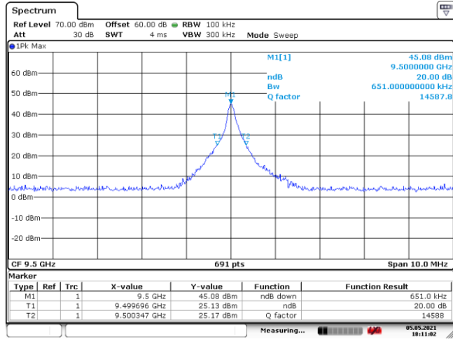
Figure 8.3-5: 20dB bandwidth, tx on mid channel with sweeping turned off
