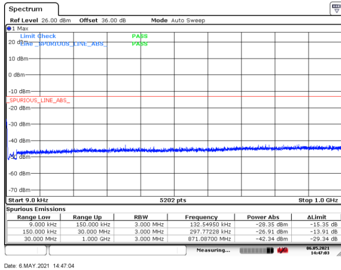
Figure 8.4-4: Conducted spurious emissions below 1 GHz, Tx on low channel
