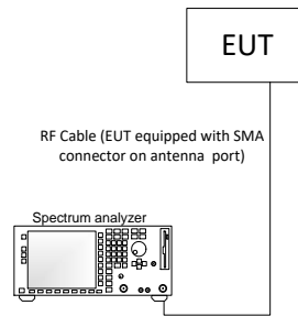
Figure 5.5-2: Antenna port testing block diagram
