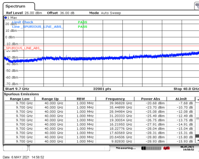
Figure 8.4-12: Conducted spurious emissions 9.7 to 40 GHz, Tx on high channel
