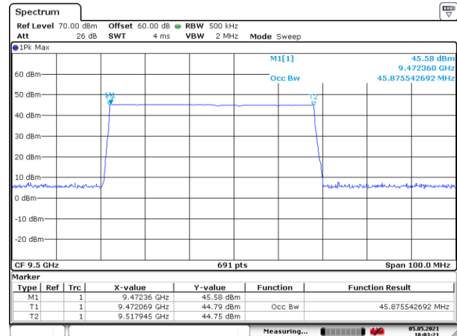
Figure 8.3-8: 99% bandwidth, tx on mid channel with sweeping turned on
