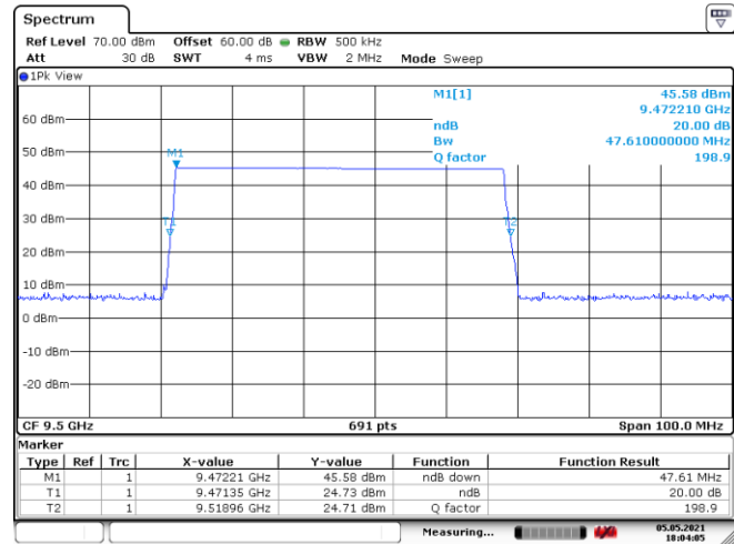
Figure 8.3-11: 20dB bandwidth, tx on mid channel with sweeping turned on
