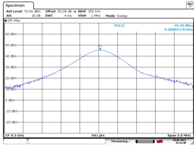
Figure 8.2-2: Output power, Tx on mid channel
