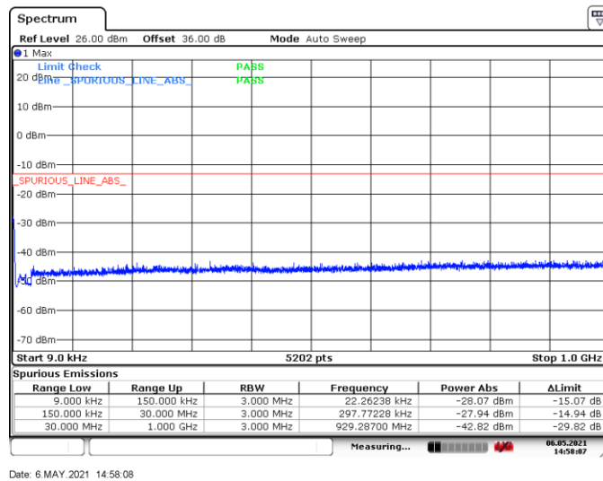
Figure 8.4-6: Conducted spurious emissions below 1 GHz, Tx on high channel
