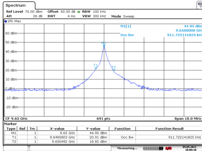
Figure 8.3-3: 99% bandwidth, tx on high channel with sweeping turned off
