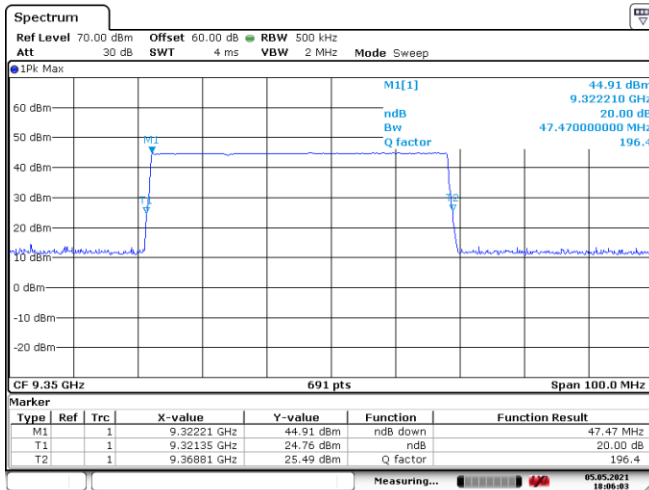
Figure 8.3-10: 20dB bandwidth, tx on low channel with sweeping turned on
