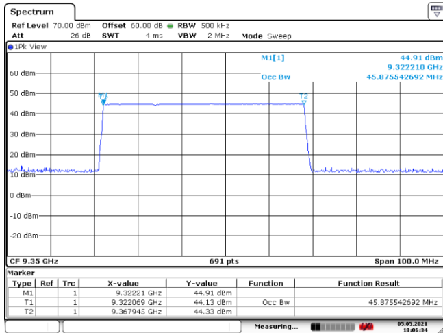
Figure 8.3-7: 99% bandwidth, tx on low channel with sweeping turned on
