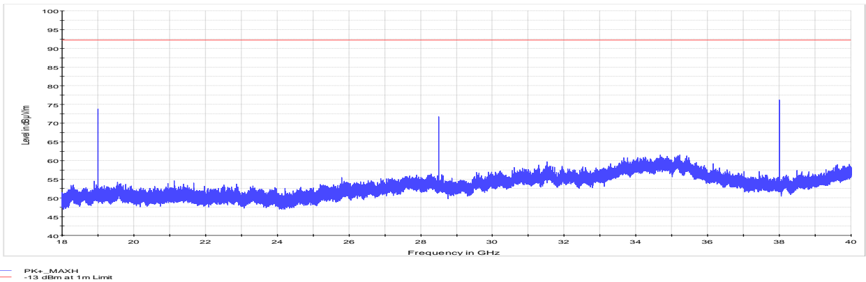
Figure 8.5-8: Cabinet radiated Spurious emissions 18 to 40 GHz, Tx @ mid channel
