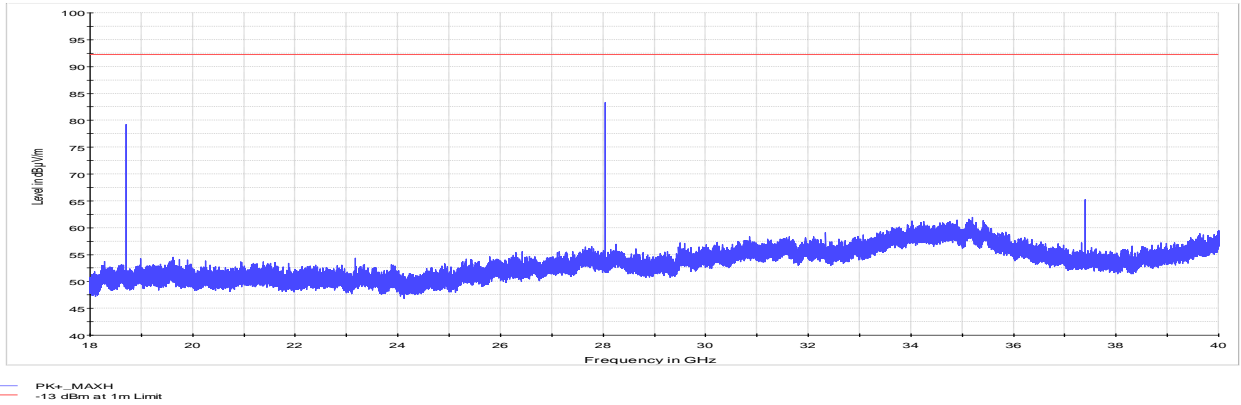
Figure 8.5-7: Cabinet radiated Spurious emissions 18 to 40 GHz, Tx @ low channel
