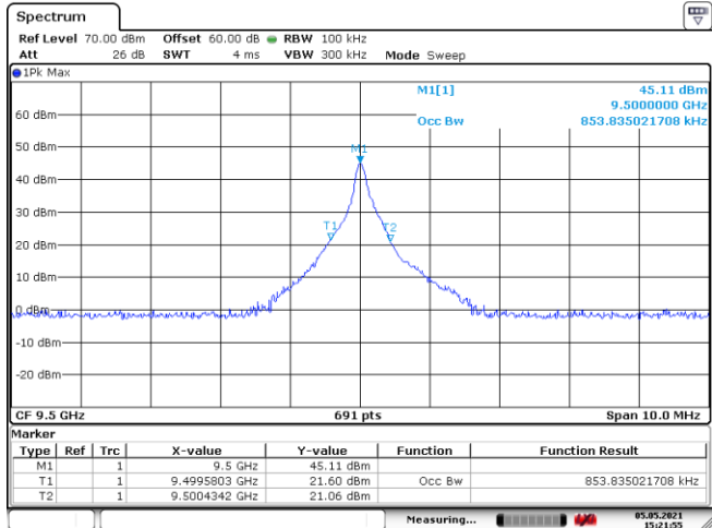
Figure 8.3-2: 99% bandwidth, tx on mid channel with sweeping turned off
