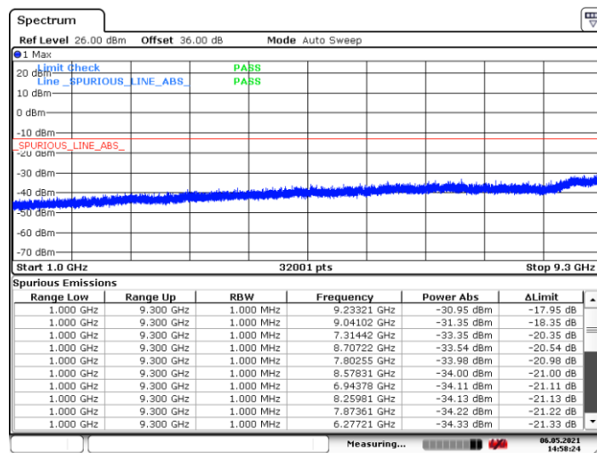
Figure 8.4-9: Conducted spurious emissions 1 to 9.3 GHz, Tx on high channel
