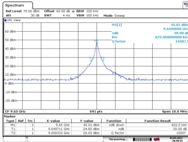
Figure 8.3-6: 20dB bandwidth, tx on high channel with sweeping turned off
