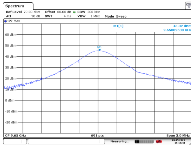
Figure 8.2-3: Output power, Tx on high channel
