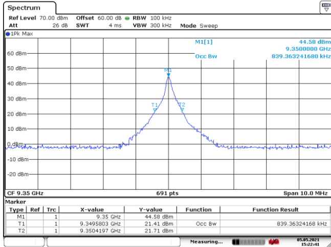
Figure 8.3-1: 99% bandwidth, tx on low channel with sweeping turned off
