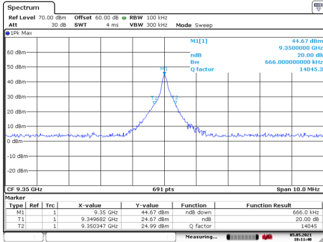
Figure 8.3-4: 20dB bandwidth, tx on low channel with sweeping turned off
