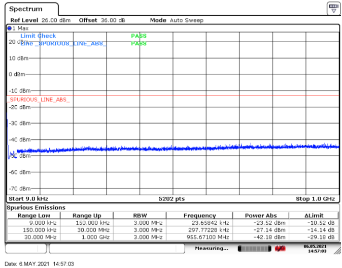
Figure 8.4-5: Conducted spurious emissions below 1 GHz, Tx on mid channel
