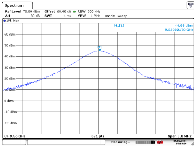
Figure 8.2-1: Output power, Tx on low channel
