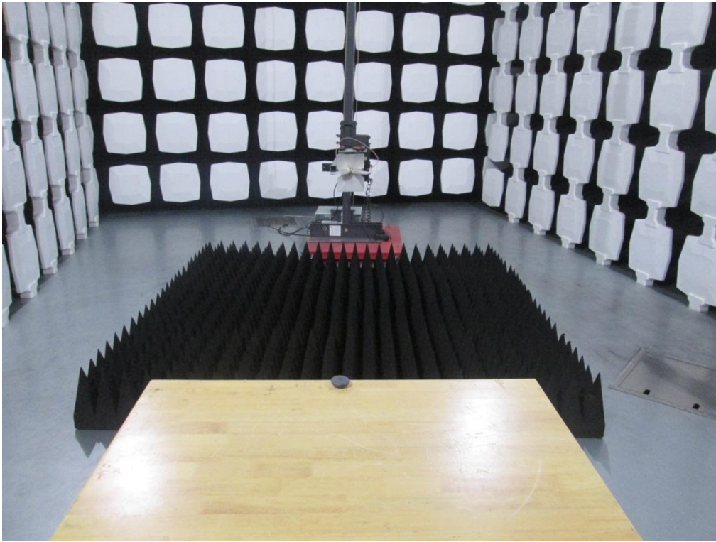
Figure 2 Radiated emission test setup (above 1 GHz)
