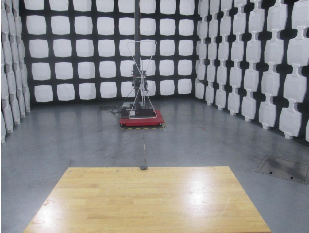
Figure 1 Radiated emission test setup (below 1 GHz)
