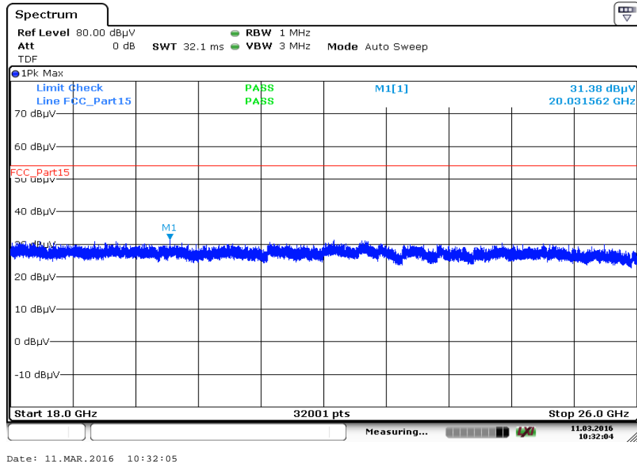
Plot 6: middle channel, 18 GHz to 26 GHz, TX mode, vertical & horizontal polarization
