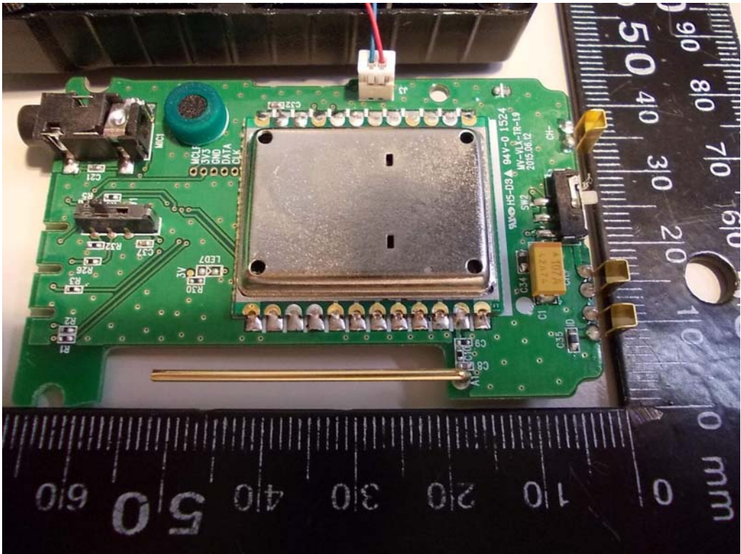
7. Front view of PCB
