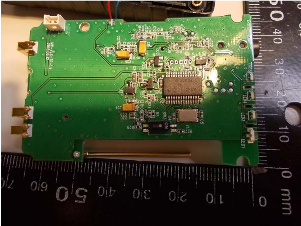
8. Rear view of PCB
