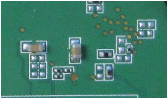
Without resistor(R2AS213)
