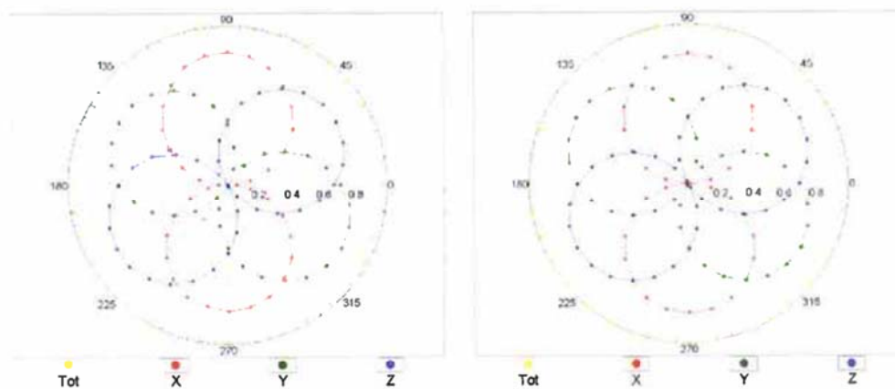
f=600 MHz,TEM
