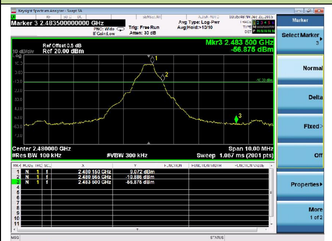
Channel 78 (2480MHz)
