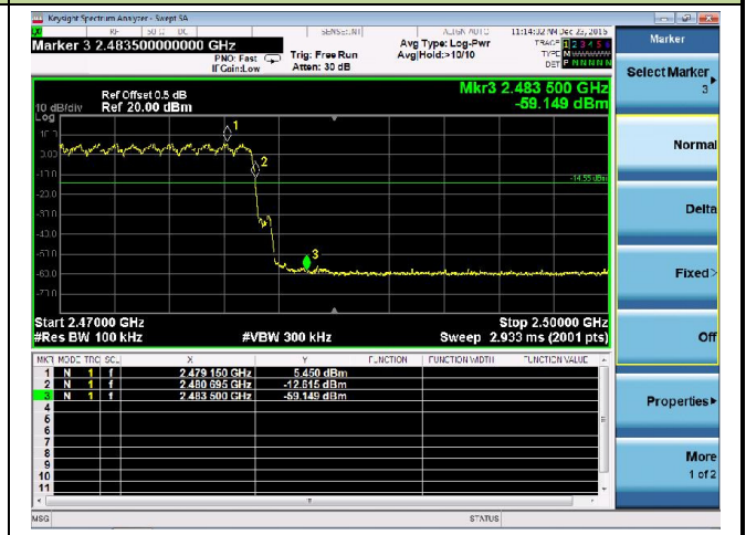
Channel 78 (2480MHz)
