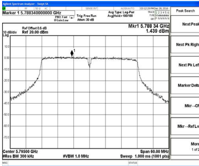
Channel 159 / 5795 MHz
