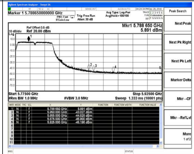
Channel 159 / 5795 MHz – Peak
