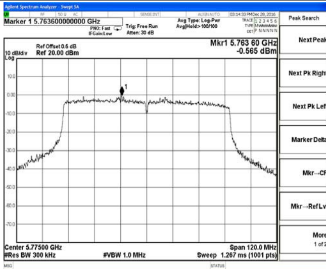
Channel 155 / 5775 MHz
