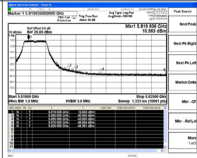
Channel 165 / 5825 MHz – Peak
