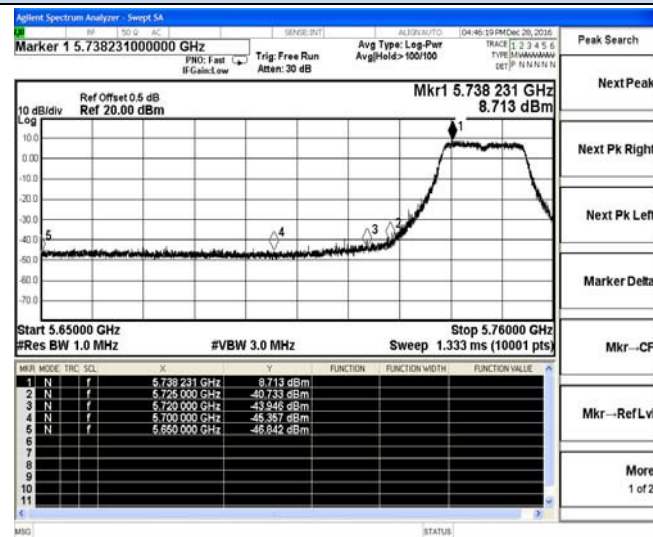
Channel 149 / 5745 MHz – Peak
