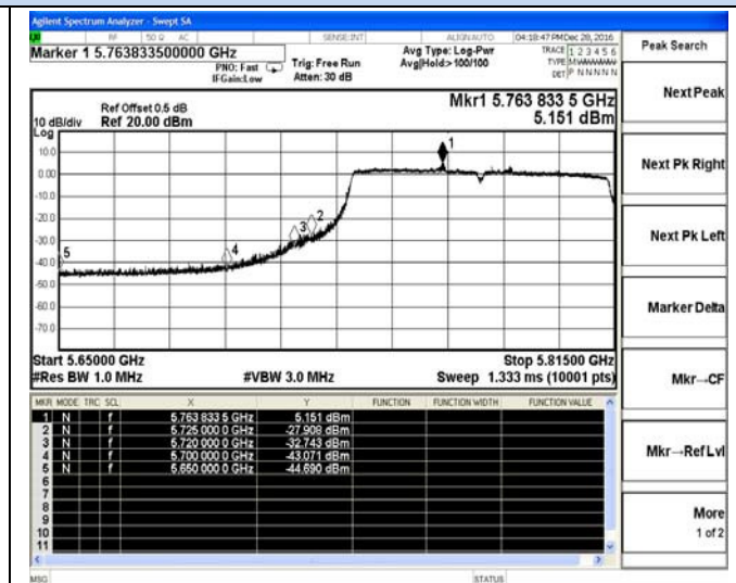
Channel 155 / 5775 MHz – Peak
