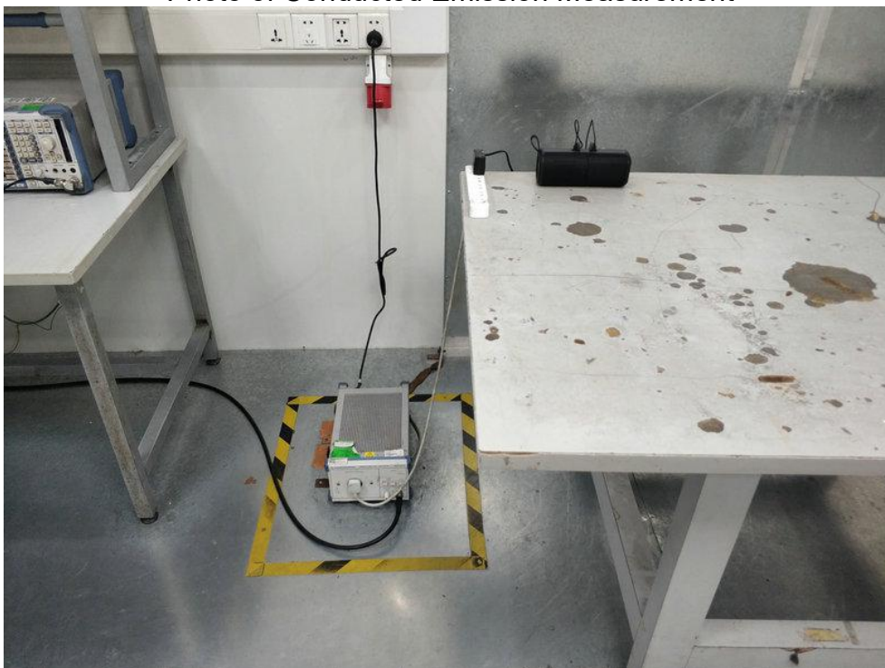
FCC ID:2AEX7-SOUNDCUP-Q Photo of Conducted Emission Measurement
