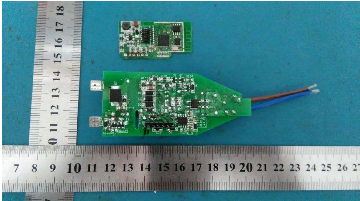
EUT- PCB Board Uncover View
