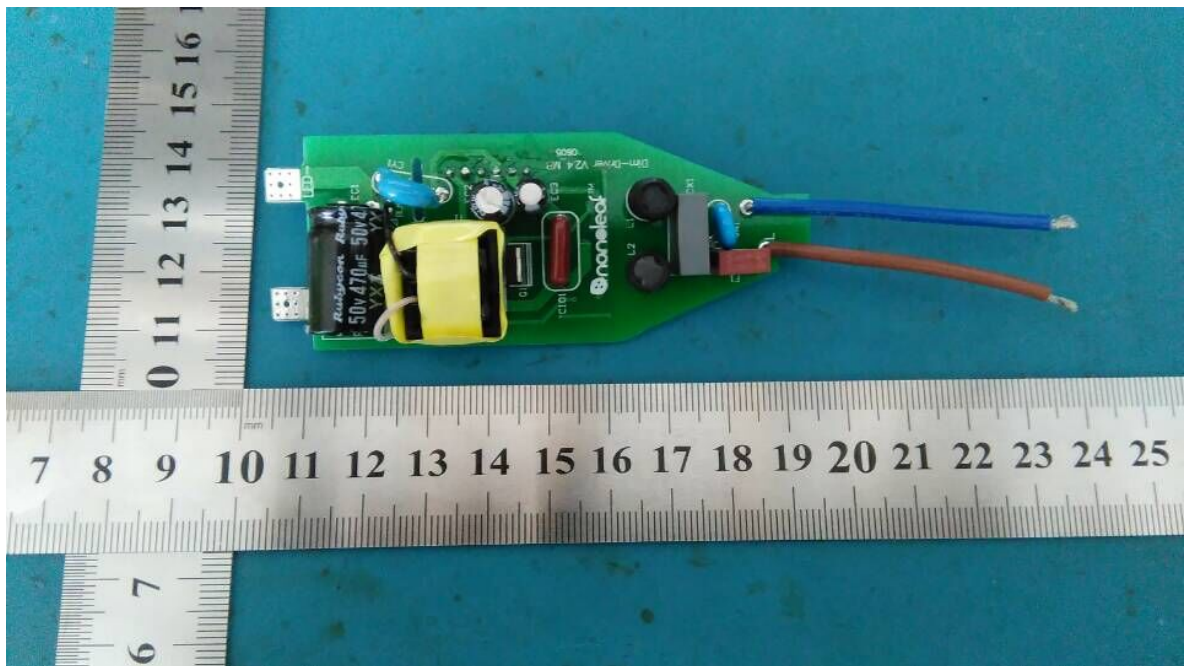
EUT- Power Board Top view
