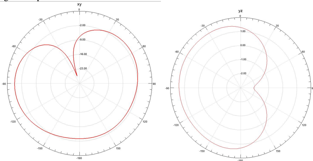
Fig.2: The pattern of the PCB Antenna
