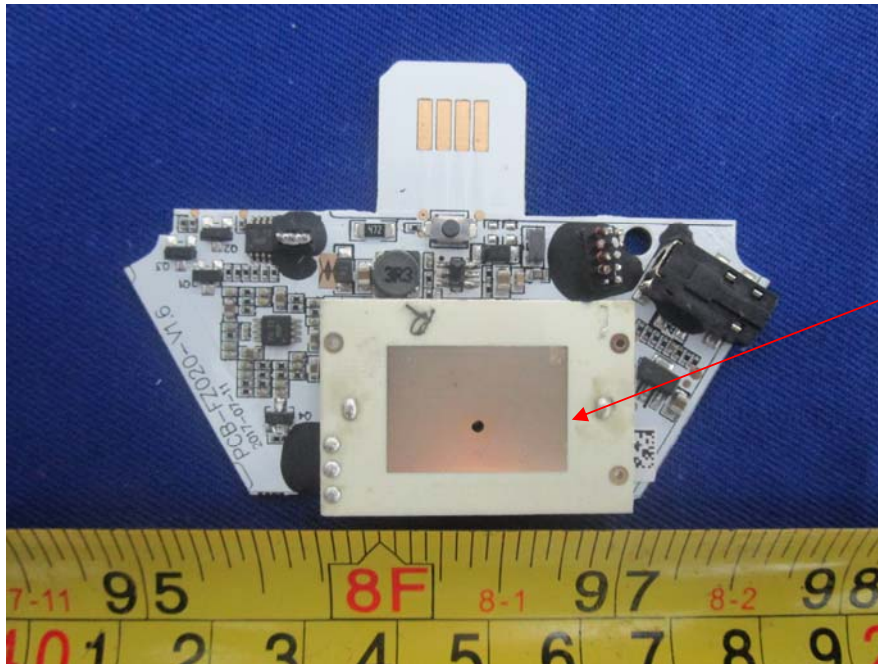
EUT -PCB-FZ020 Top View
