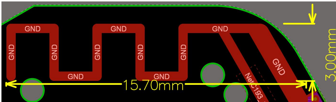
Fig.1: The dimension of the PCB Antenna
