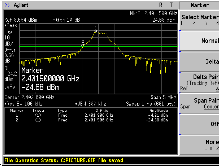
Channel 00 (2402MHz)
