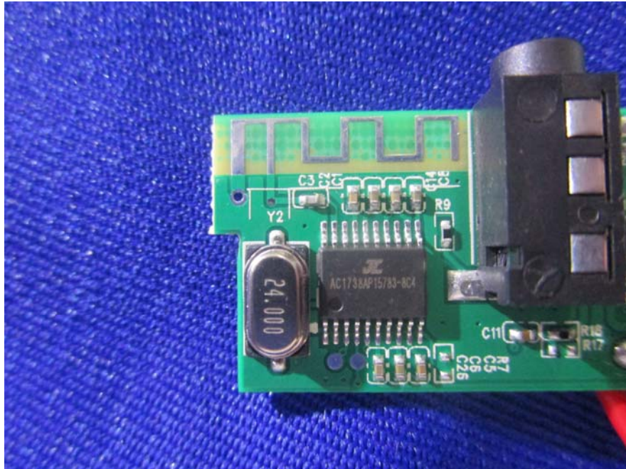
EUT – Chip&Ant View
