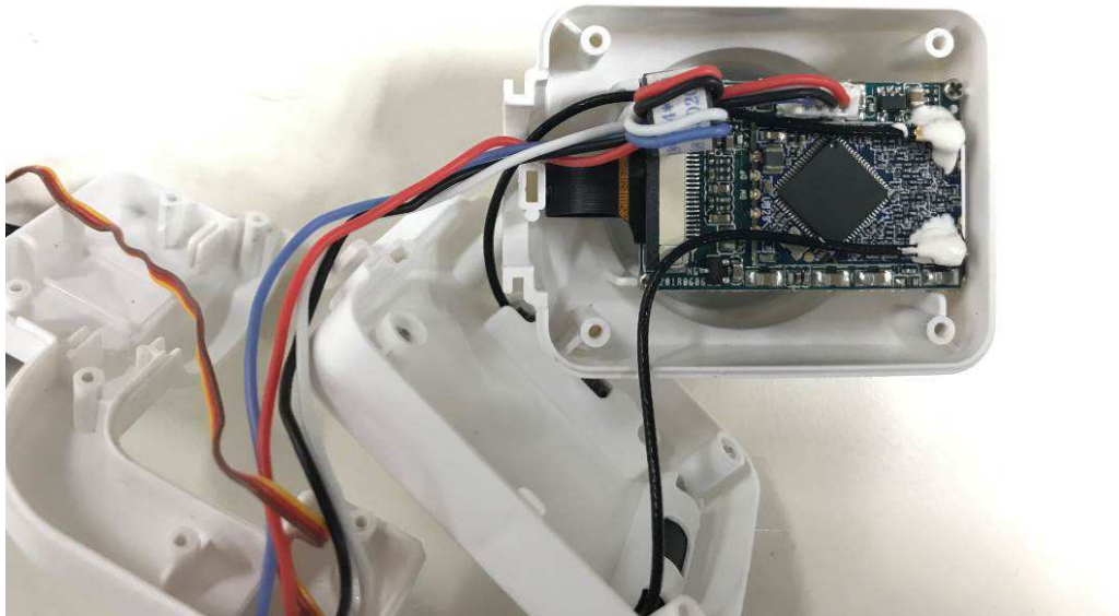
Internal View
