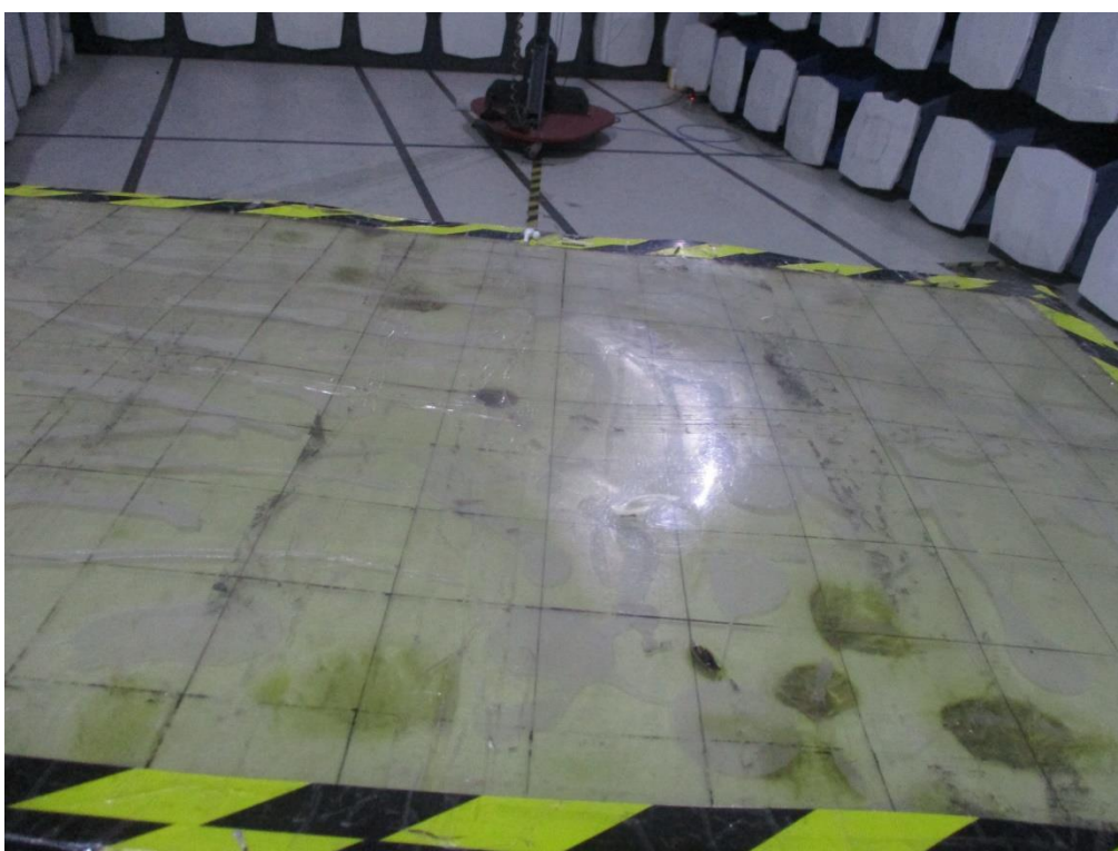
Up to 1GHz - EUT is on the center of the turn table
