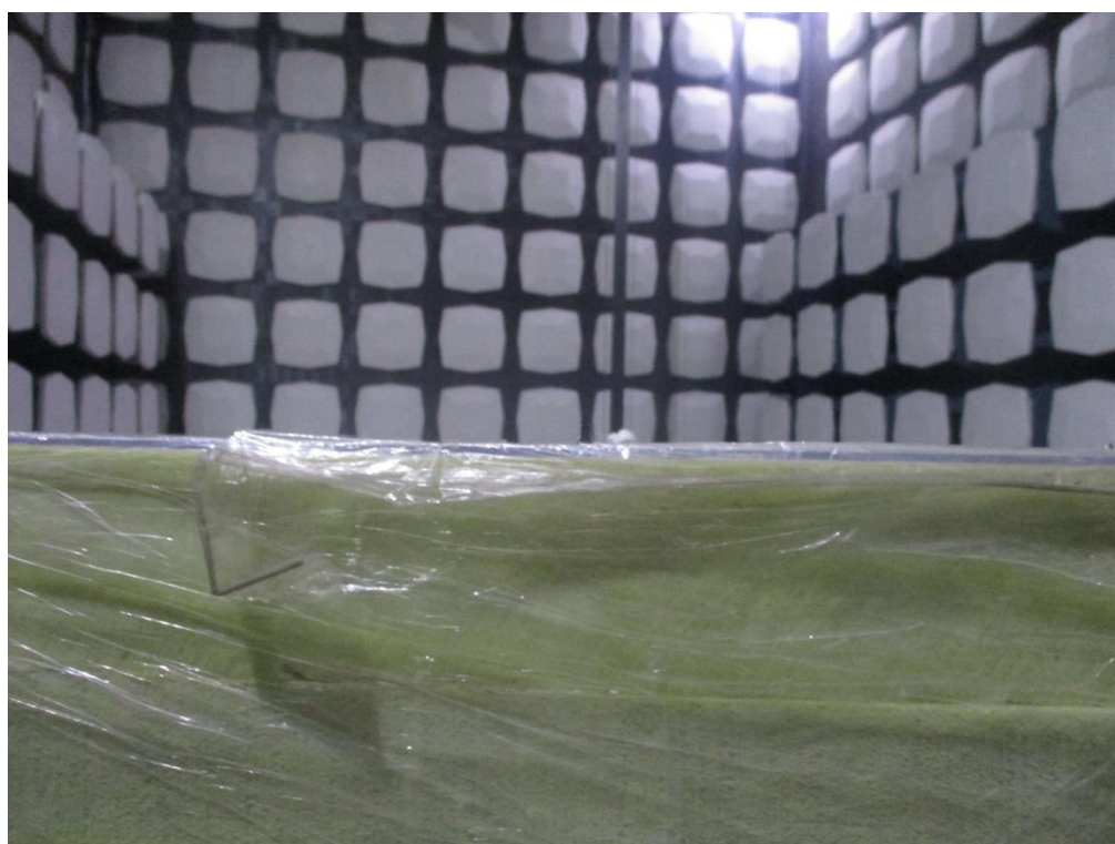
Above 1GHz - EUT is on the center of the turn table
