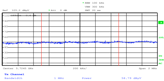
Figure 8.1-1: Radiated – Undesirable (unwanted) emissions at lower band edge peak, (Channel 149 – 5745 MHz)
