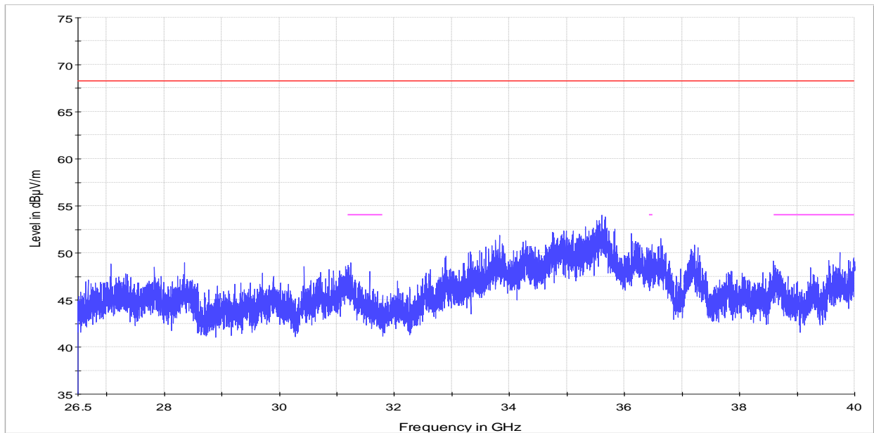
Figure 8.1-13: Radiated – Undesirable (unwanted) emissions 26 to 40 GHz, Channel 157 – 5785 MHz
