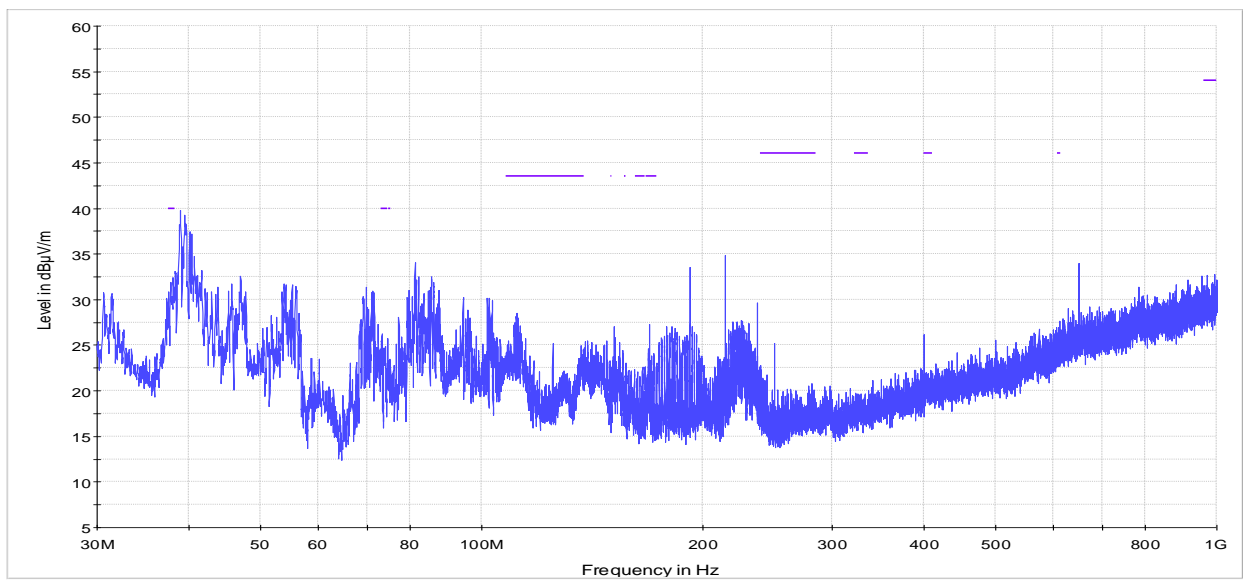
Figure 8.1-4: Radiated – Undesirable (unwanted) emissions below 1 GHz, Channel 157 – 5785 MHz
