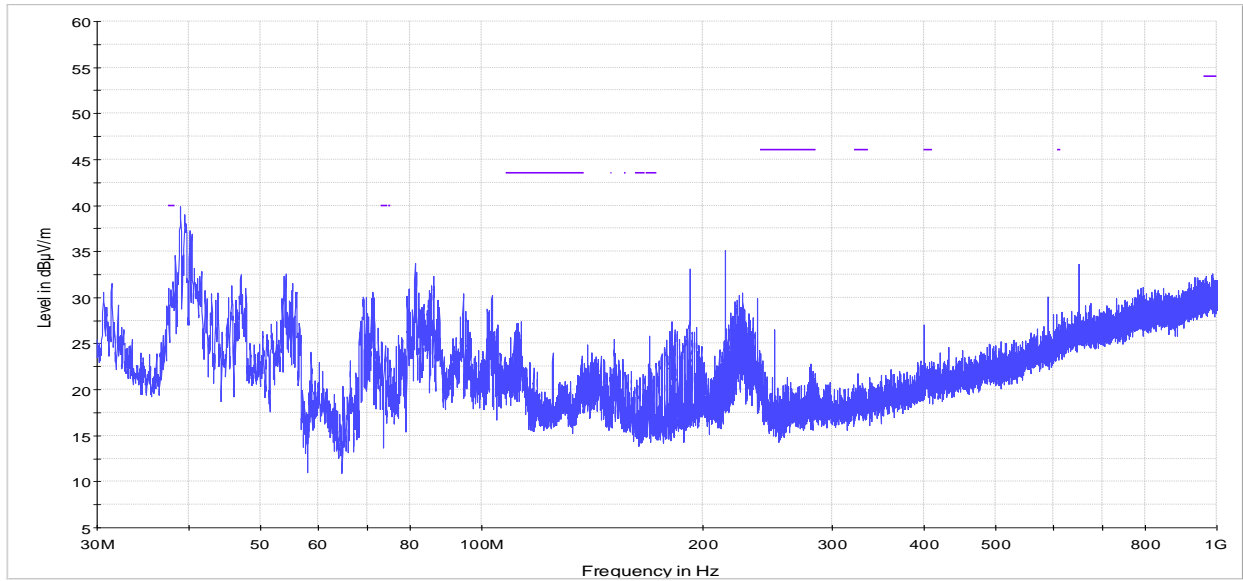
Figure 8.1-3: Radiated – Undesirable (unwanted) emissions below 1 GHz, Channel 149 – 5745 MHz
