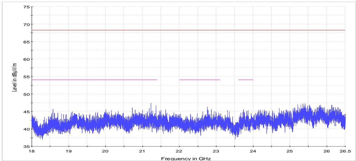
Figure 8.1-9: Radiated – Undesirable (unwanted) emissions 18 to 26 GHz, Channel 149 – 5745 MHz
