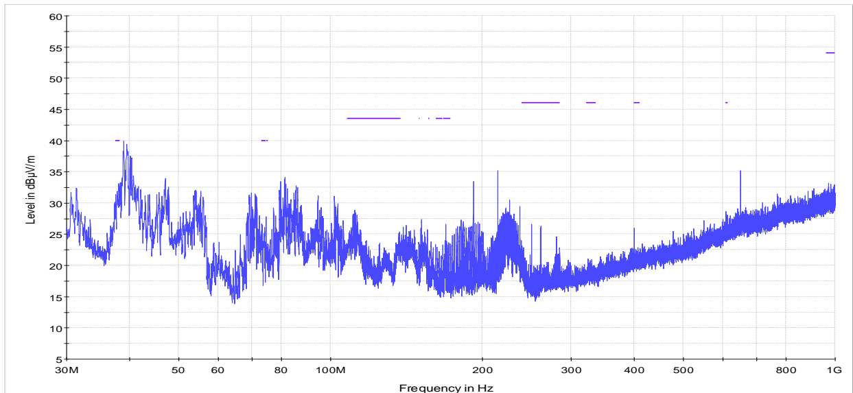
Figure 8.1-4: Radiated – Undesirable (unwanted) emissions below 1 GHz, Channel 116 – 5580 MHz
