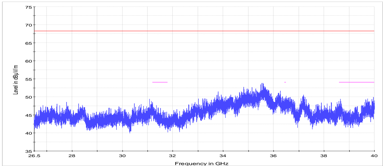
PK+_MAXH 68.23 dBuV (-27 dBm) 3m Peak Limit (Outside restricted Bands) FCC 15.205 and RSS-Gen Restricted bands limits
