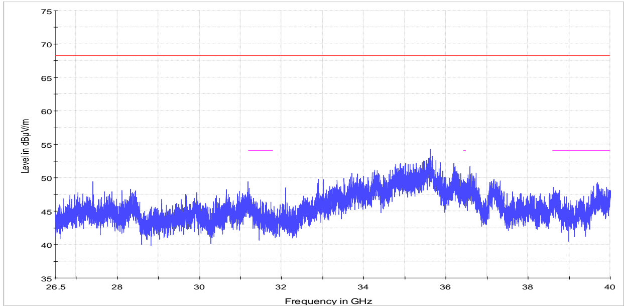
PK+_MAXH 68.23 dBuV (-27 dBm) 3m Peak Limit (Outside restricted Bands) FCC 15.205 and RSS-Gen Restricted bands limits
