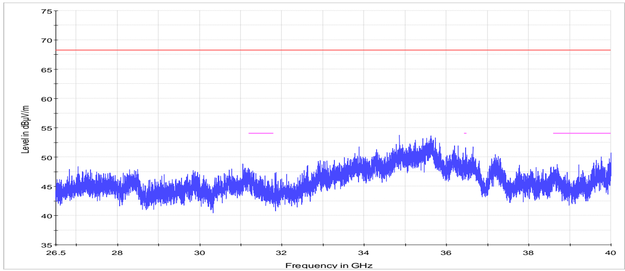
— PK+_MAXH — 68.23 dBµV (-27 dBm) 3m Peak Limit (Outside restricted Bands) — FCC 15.205 and RSS-Gen Restricted bands limits
