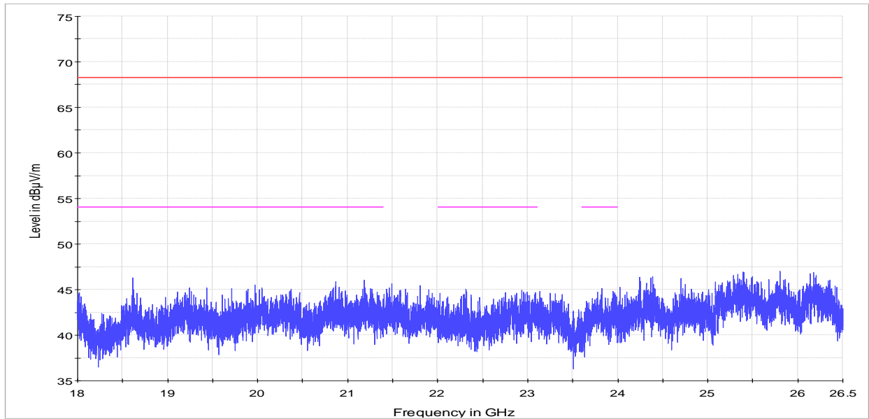
— PK+_MAXH — 68.23 dBµV (-27 dBm) 3m Peak Limit (Outside restricted Bands) — FCC 15.205 and RSS-Gen Restricted bands limits
