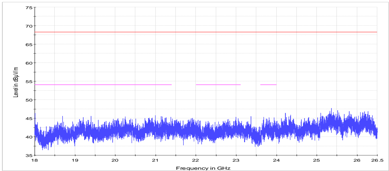
Figure 8.1-9: Radiated – Undesirable (unwanted) emissions 18 to 26 GHz, Channel 100 – 5500 MHz
