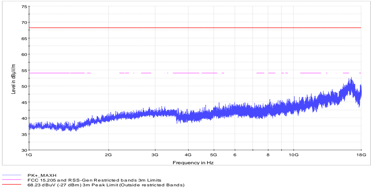
Figure 8.1-7: Radiated – Undesirable (unwanted) emissions 1 to 18 GHz, Channel 116 – 5580 MHz
