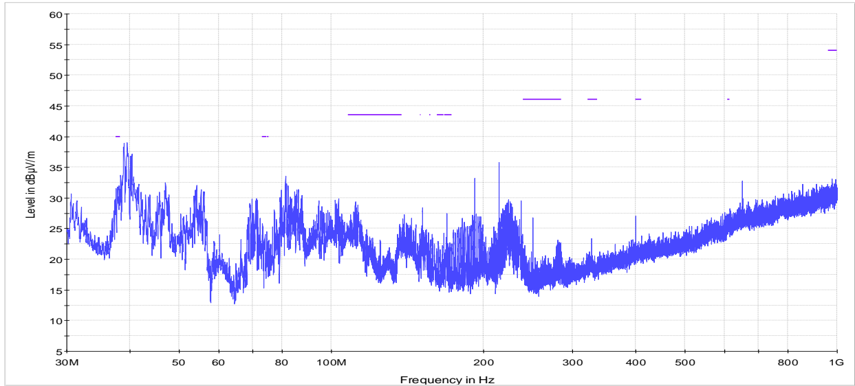
Figure 8.1-3: Radiated – Undesirable (unwanted) emissions below 1 GHz, Channel 100 – 550 MHz
