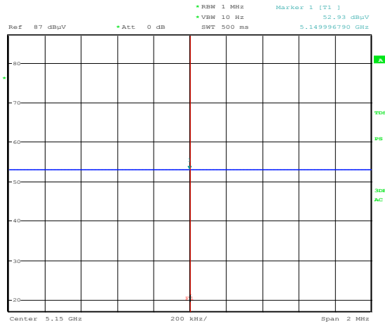
Figure 8.1-2: Radiated – Undesirable (unwanted) emissions within restricted band at 5.15 GHz, Average (Channel 36 – 5180 MHz)
