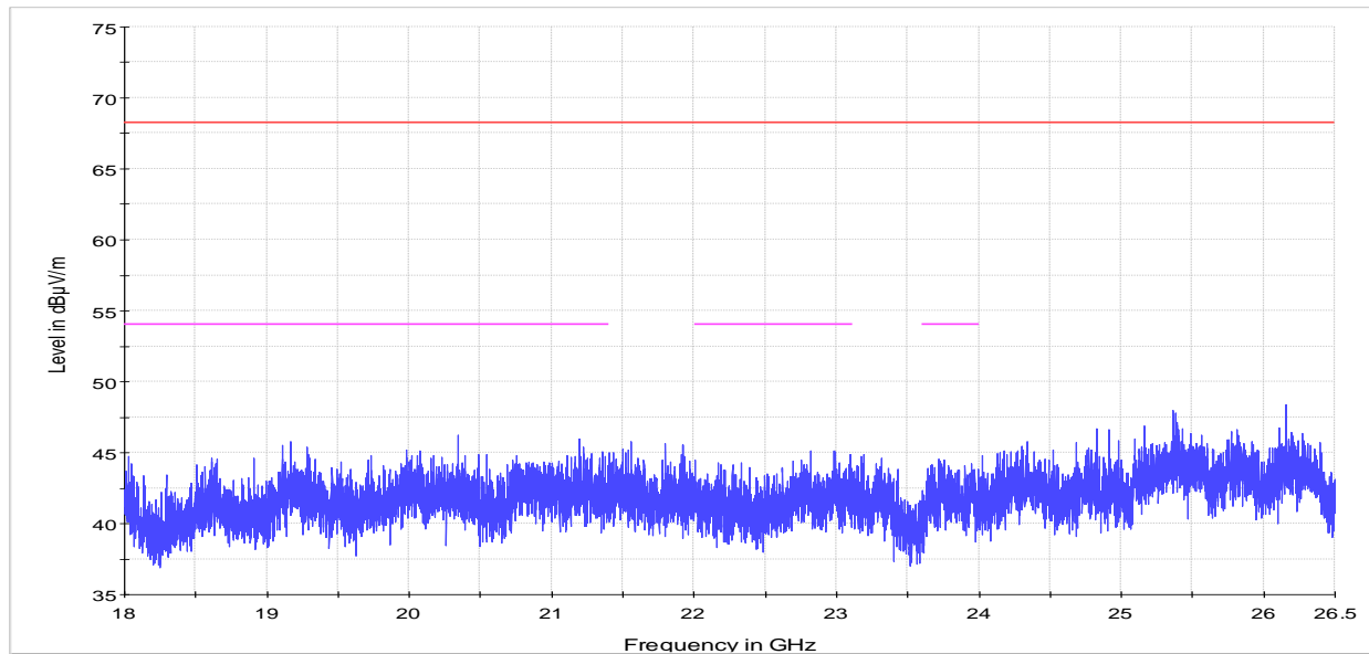
Figure 8.1-10: Radiated – Undesirable (unwanted) emissions 18 to 26 GHz, Channel 36 – 5180 MHz
