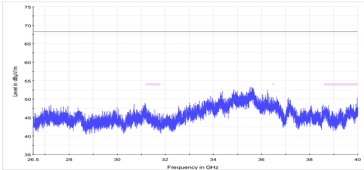
Figure 8.1-14: Radiated – Undesirable (unwanted) emissions 26 to 40 GHz, Channel 44 – 5220 MHz
