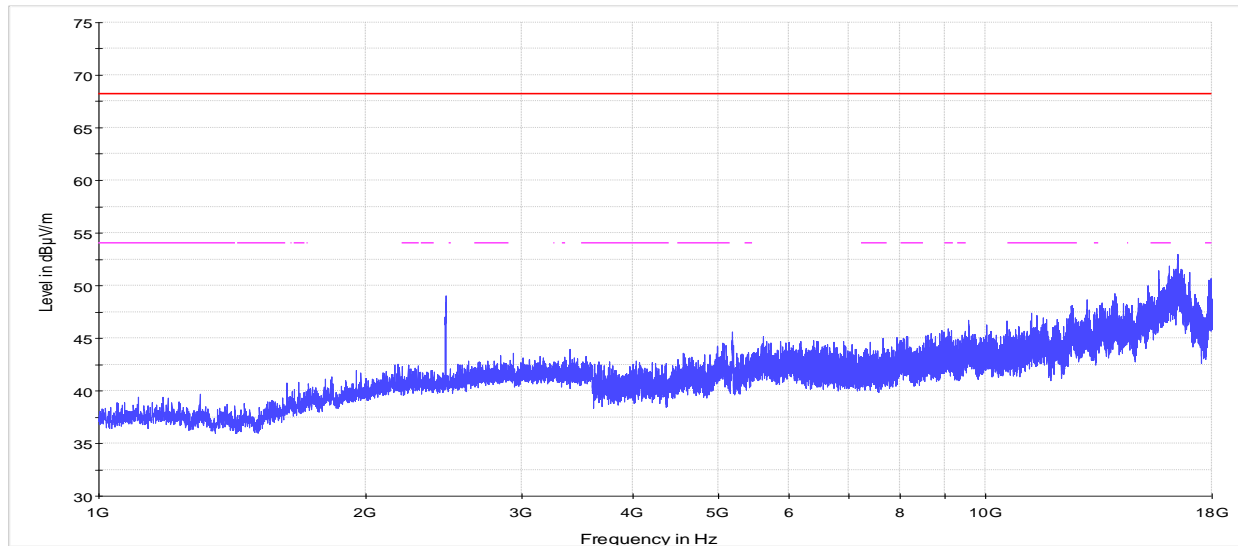
PK+_MAXH FCC 15.205 and RSS-Gen Restricted bands 3m Limits 68.23 dBuV (-27 dBm) 3m Peak Limit (Outside restricted Bands)
