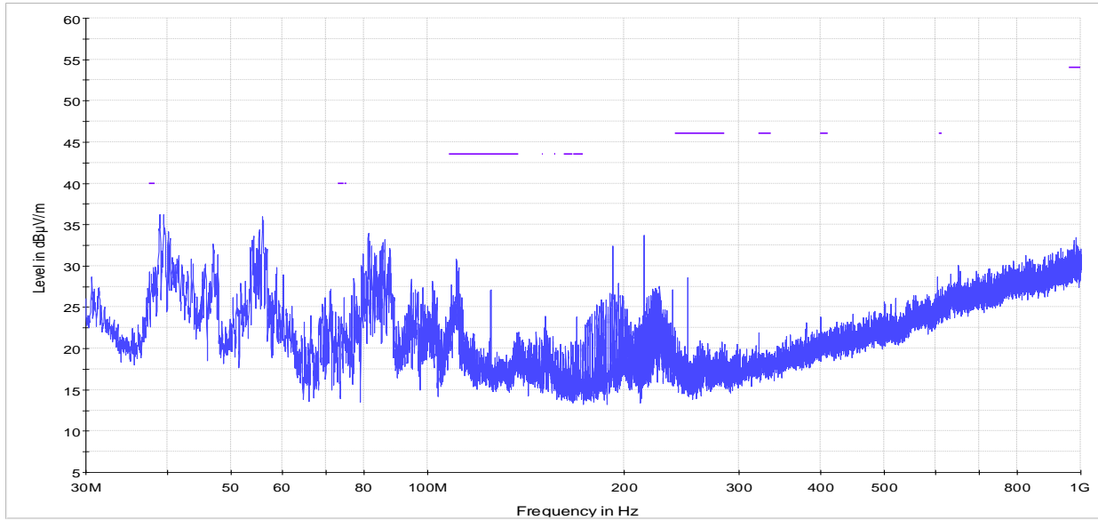
PK+_MAXH FCC 15.205 and RSS-Gen Restricted bands limits
