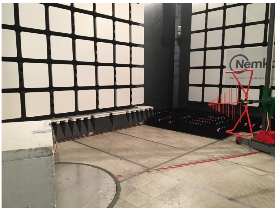
Figure 8.1-17: Radiated – Undesirable (unwanted) emissions setup photo – below 1 GHz
