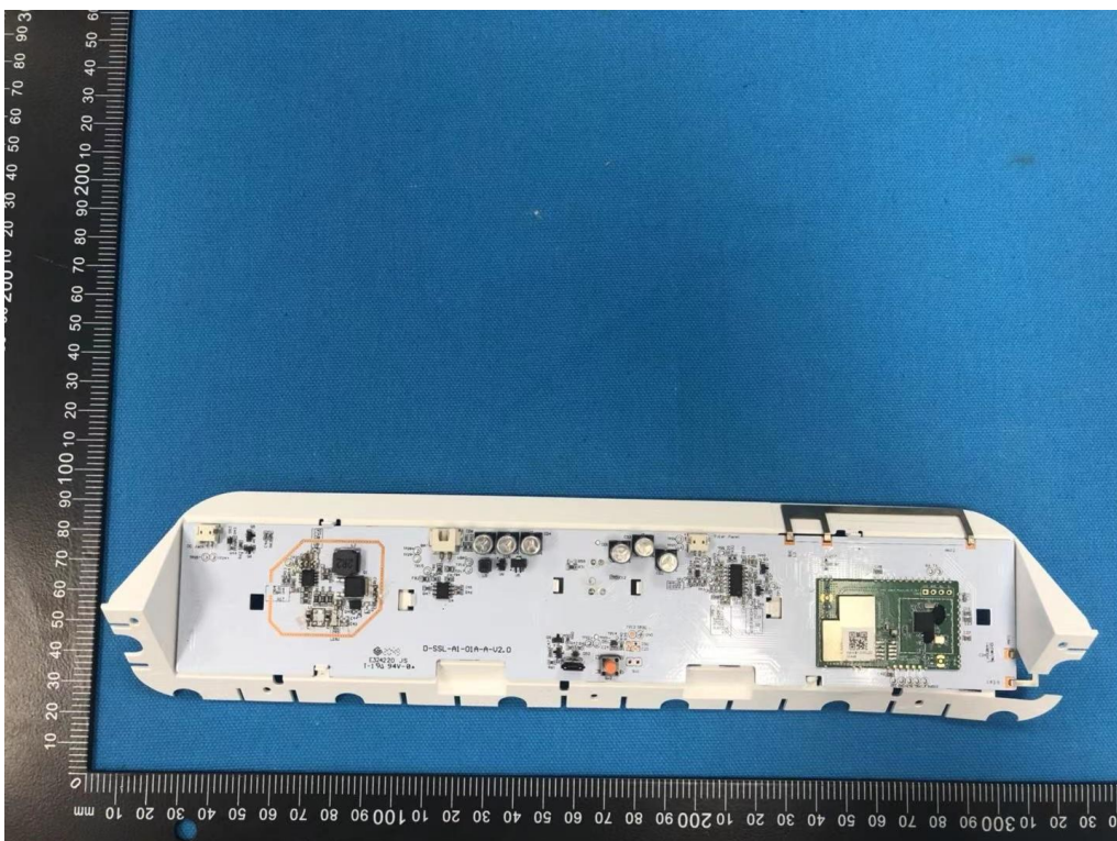
PCBA of 5D22E5
