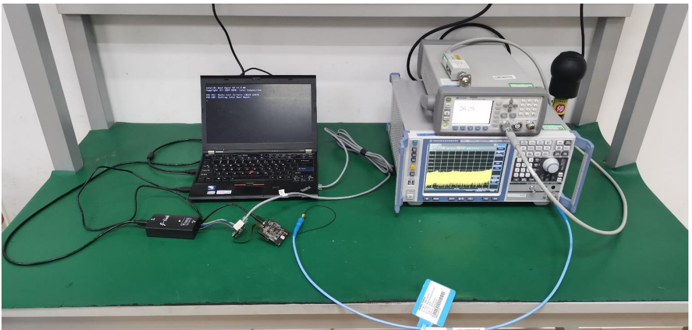
Description: Antenna port conducted test
