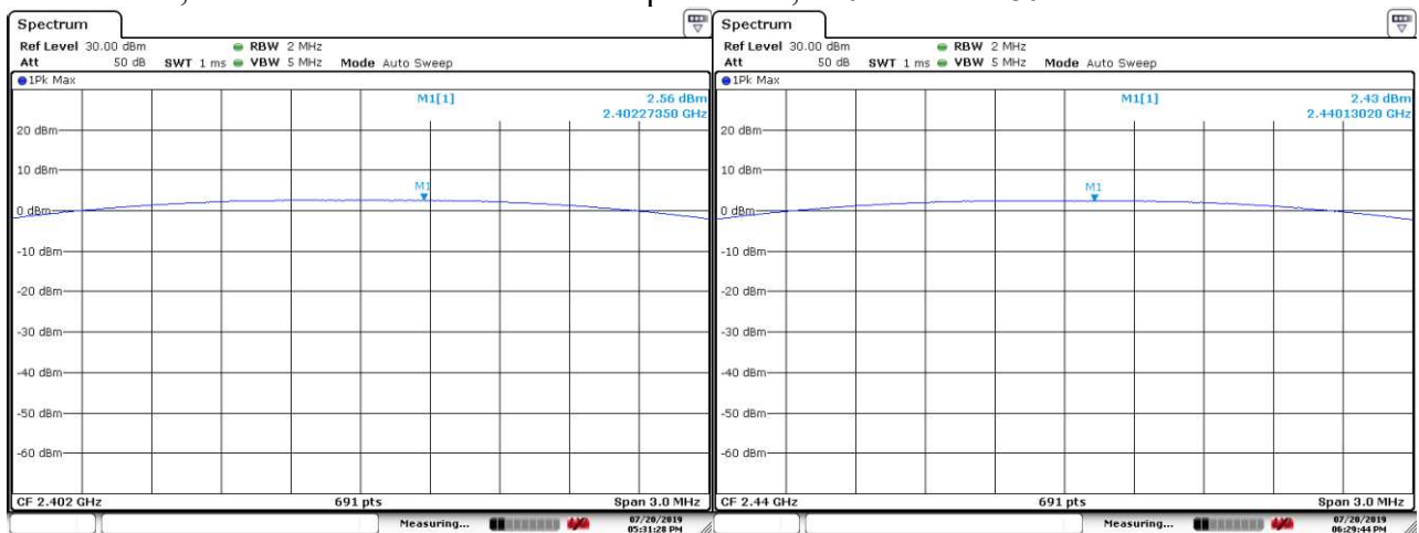
Figure 3: Maximum peak Conducted Output Power
