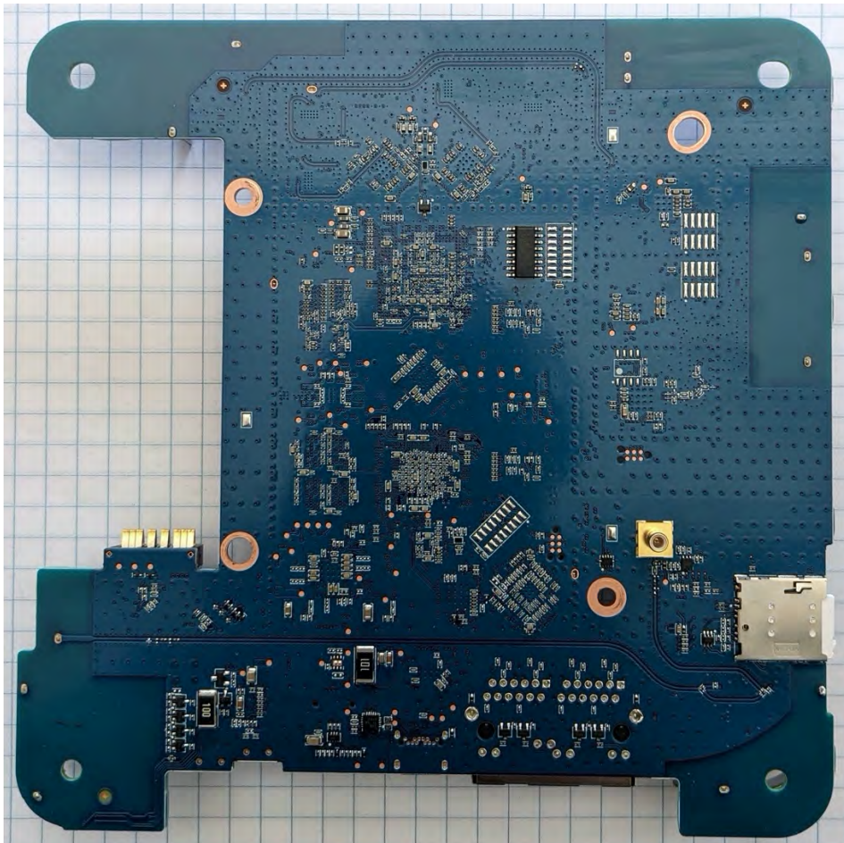
PCB below
