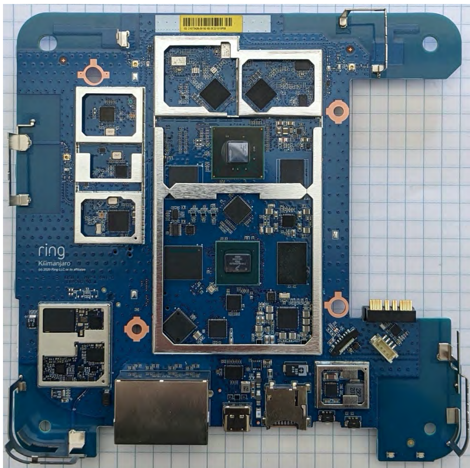
PCB above – shields removed
