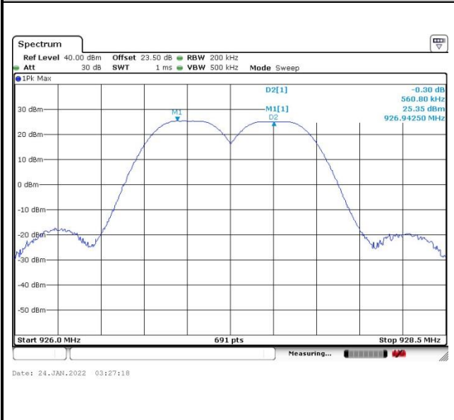
Channel Separation Plot on Channel 50 - 51
