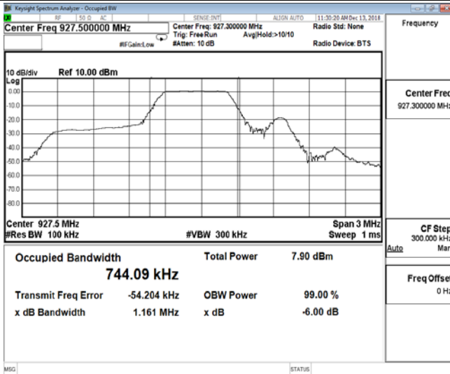
Channel 26 / 927.5 MHz
