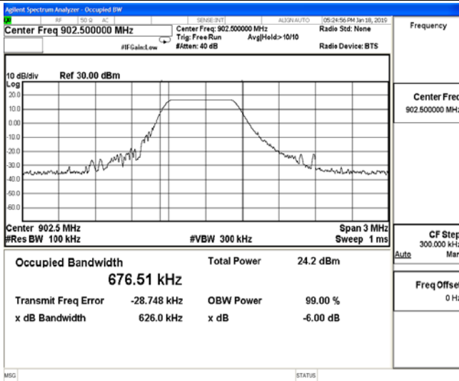
Channel 0 / 902.5 MHz
