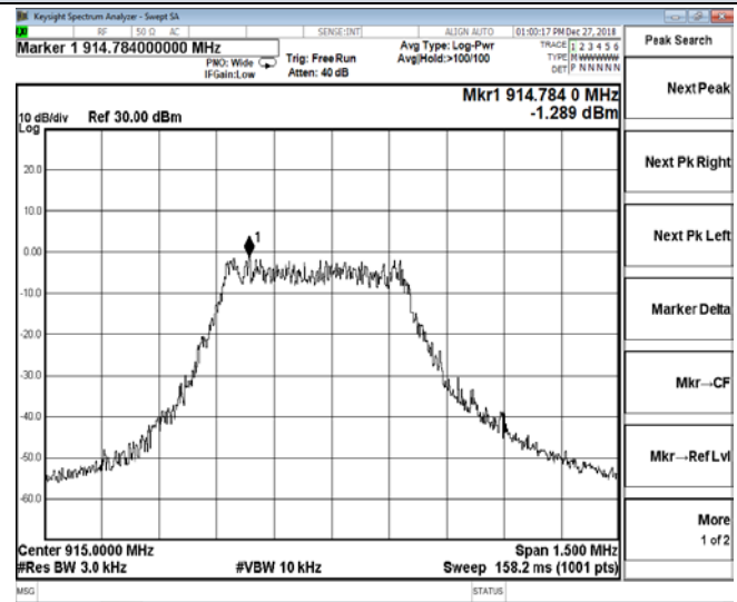
Channel 13 / 915 MHz
