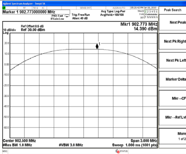
Channel 0 / 902.5 MHz
