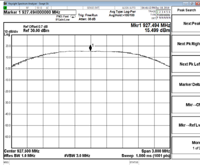
Channel 26 / 927.5 MHz
