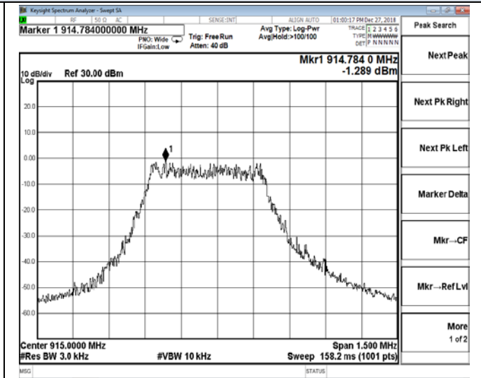
Channel 13 / 915 MHz
