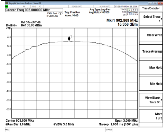
Channel 1 / 903.0 MHz
