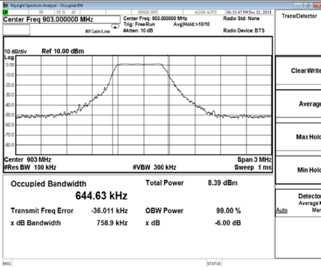
Channel 1 / 903.0 MHz
