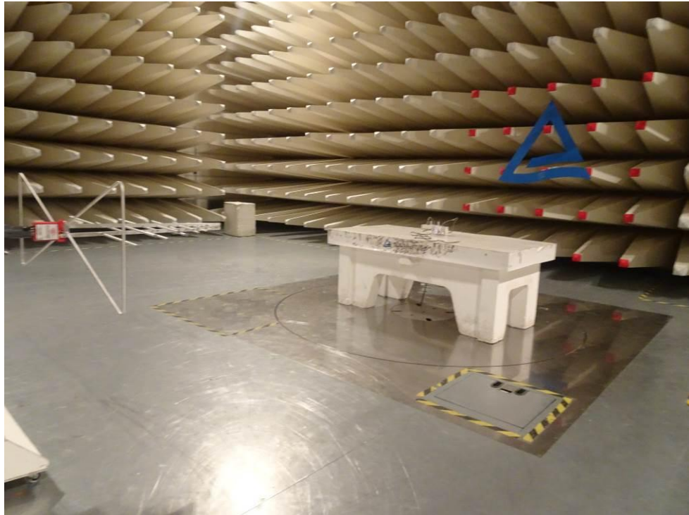
Test Setup
