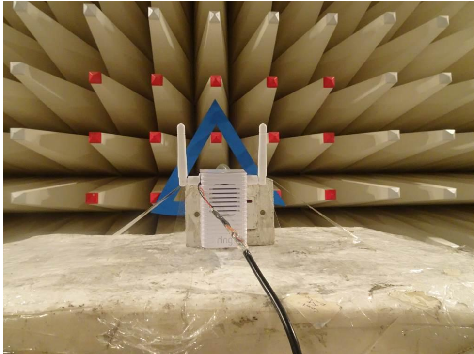
EUT on the test table
