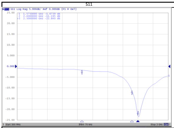
BT antenna passive data
