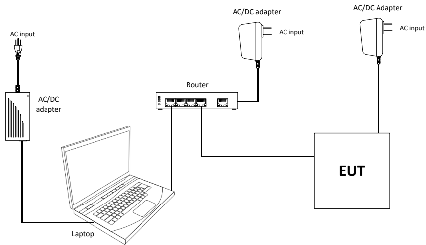
Figure 6.4-1: block diagram
