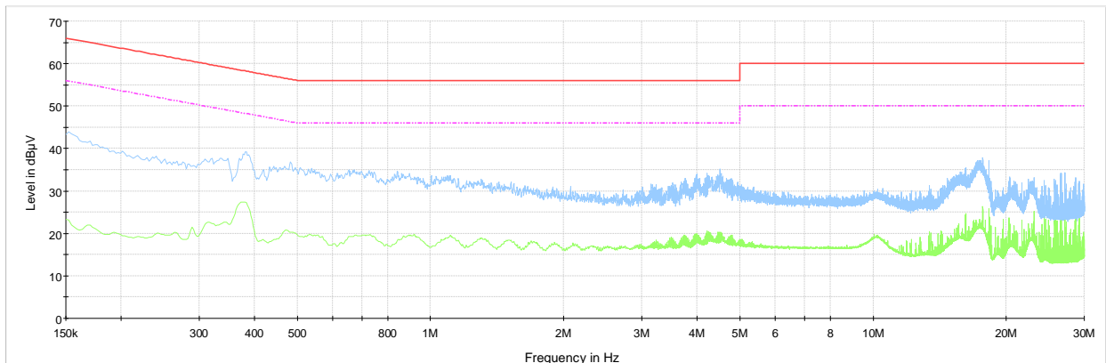
Conducted emissions 150 kHz - 30 MHz 120 Vac 60 Hz Neutral
