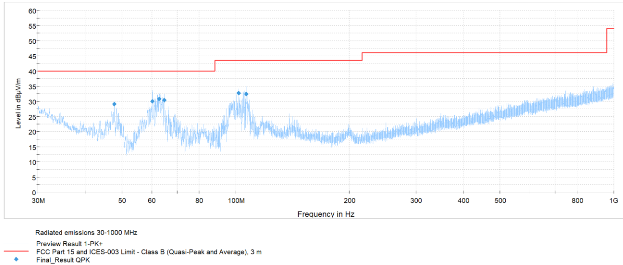
Figure 8.1-1: Radiated emissions spectral plot (30 to 1000 MHz)
