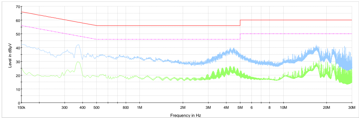
Conducted emissions 150 kHz - 30 MHz 120 Vac 60 Hz Phase
