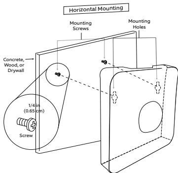
Fig. 1: Horizontal Mounting
