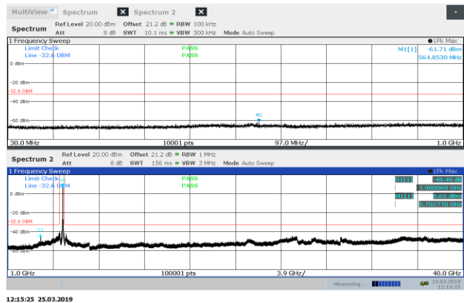
Figure 8.8-33: Conducted spurious emissions 30 MHz – 40 GHz, high channel, 802.11a
