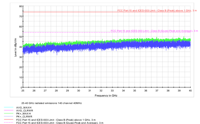
Figure 8.8-28: Radiated spurious emission 25 to 40 GHz, high channel, 802.11n
