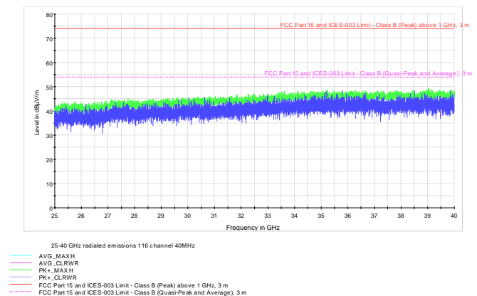
Figure 8.8-27: Radiated spurious emission 25 to 40 GHz, mid channel, 802.11n
