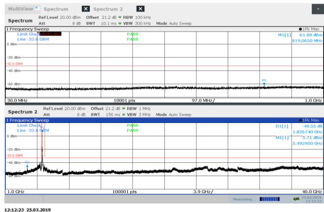
Figure 8.8-31: Conducted spurious emissions 30 MHz – 40 GHz, low channel, 802.11a
