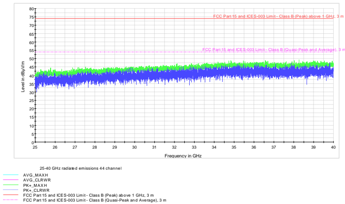
Figure 8.8-21: Radiated – Undesirable (unwanted) emissions 25 to 40 GHz, Channel 44 – 5220 MHz 802.11a
