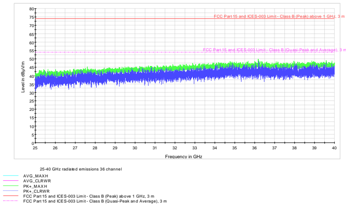
Figure 8.8-20: Radiated – Undesirable (unwanted) emissions 25 to 40 GHz, Channel 36 – 5180 MHz 802.11a
