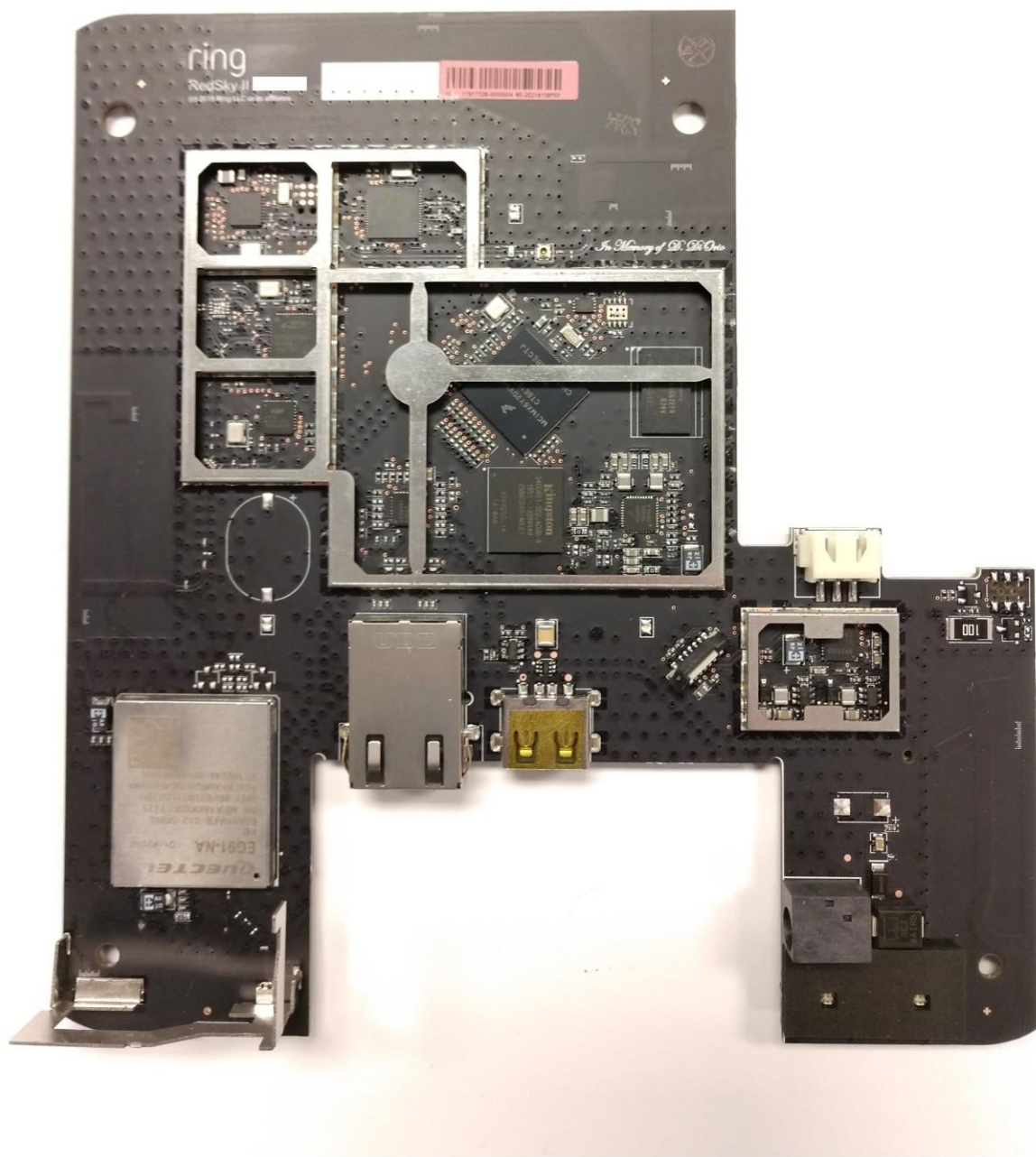
Figure 2 Top view, shielding removed
