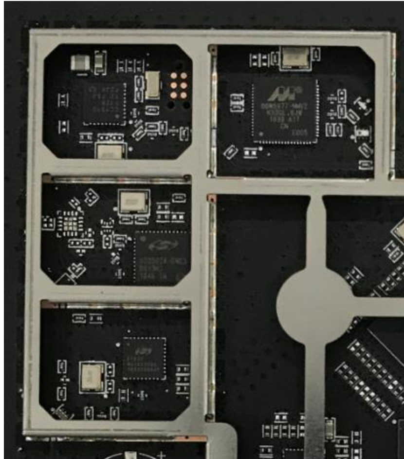
Figure 3 Location of radios
