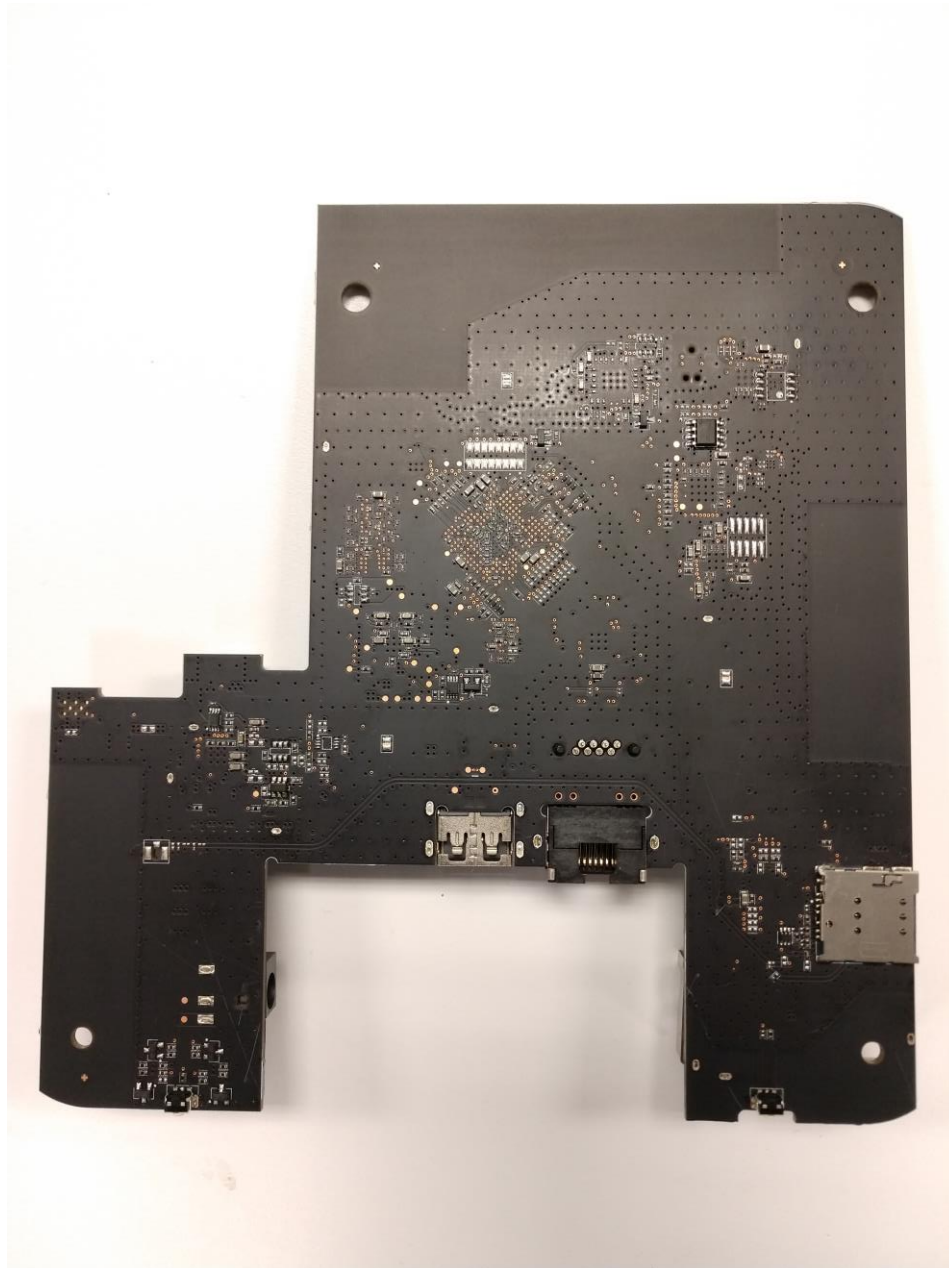
Figure 5 Underside view
