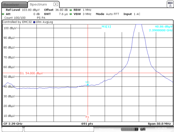
Figure 8.7-9: Radiated restricted bands spurious emissions at 2.39 GHz , average
