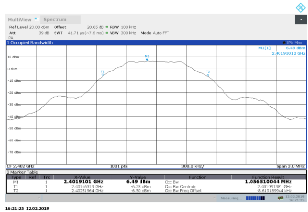
Figure 8.5-4: 99% occupied bandwidth on low channel
