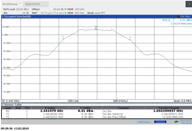
Figure 8.5-5: 99% occupied bandwidth on mid channel
