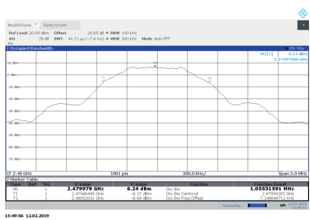
Figure 8.5-6: 99% occupied bandwidth on high channel
