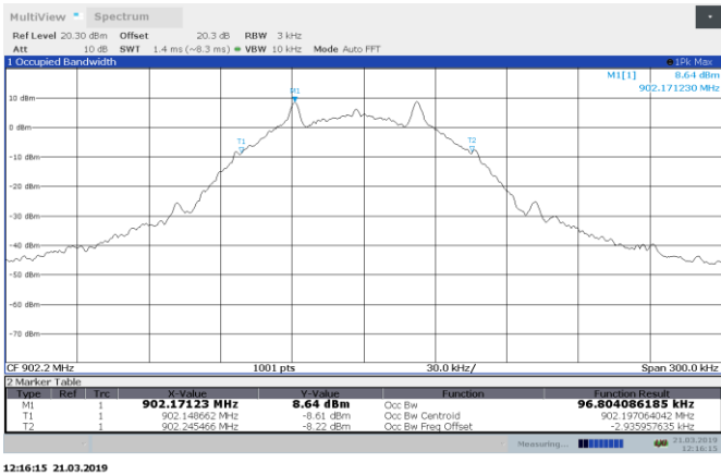
Figure 8.5-4: 99% OBW on low channel
