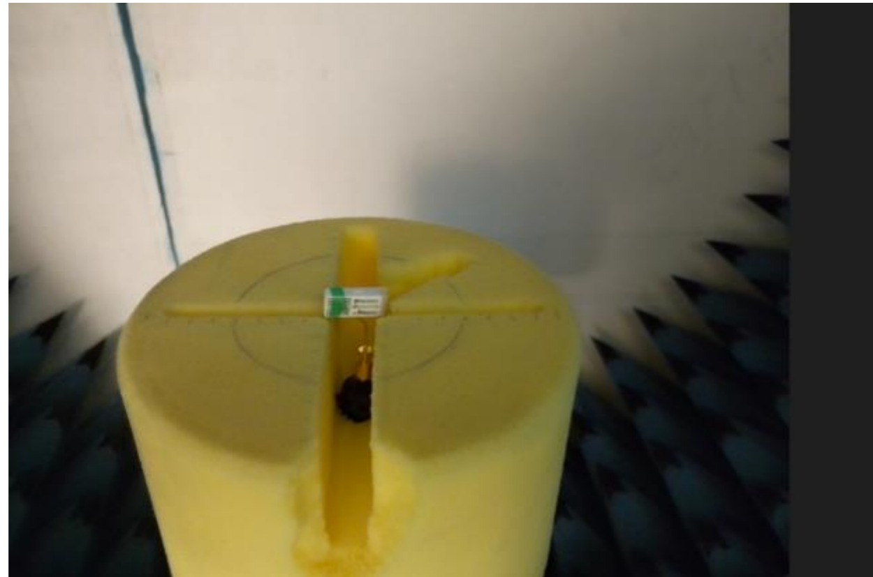
Total efficiency and max gain measurement setup:
