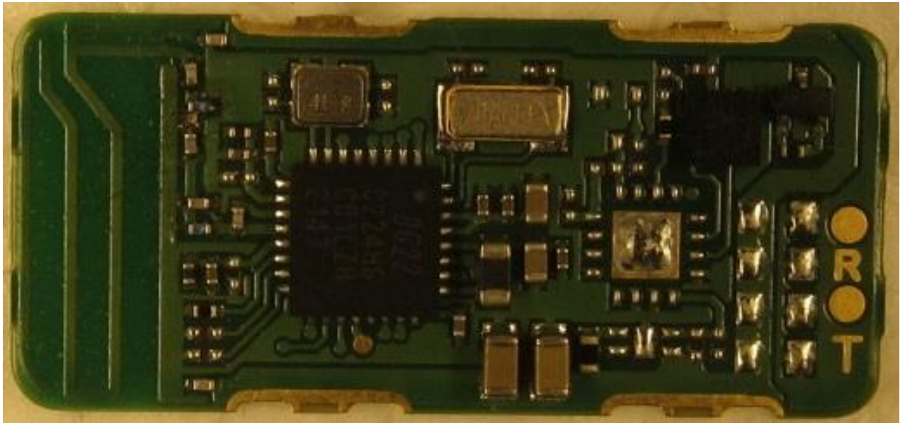
PCB Bottom:
