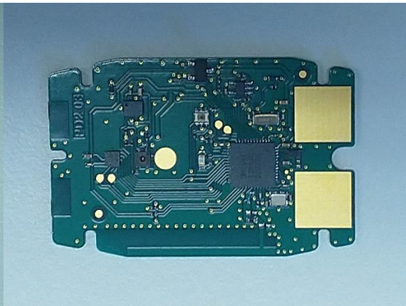
2 PWB top
