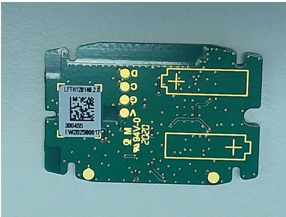
1 PWB bottom
