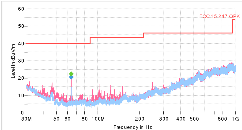
The above plot shows the results of the scan using peak detector.
